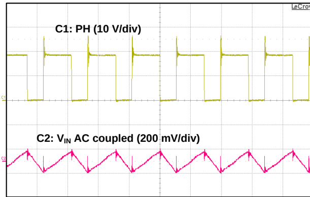
Timebase: 2.00 \mu s/div Figure 10. Input Voltage Ripple
