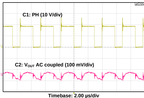
Figure 7. Maximum Load Output Voltage Ripple
