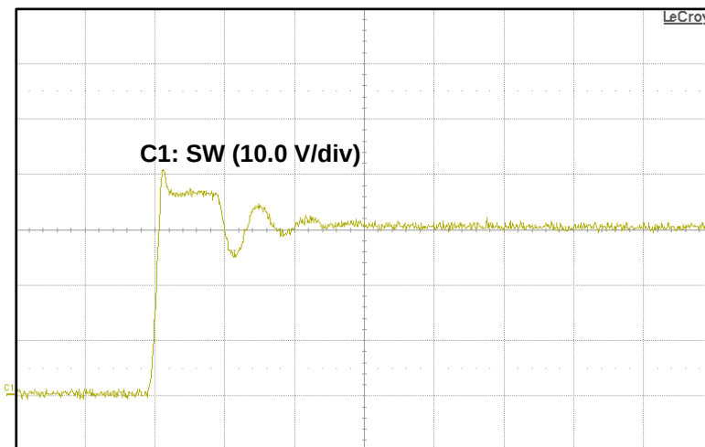
Timebase: 50 ns/div
