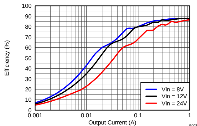
Figure 2. Light-Load Efficiency
