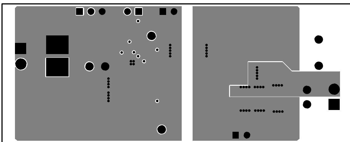
Figure 20. Internal Layer-2 Layout
