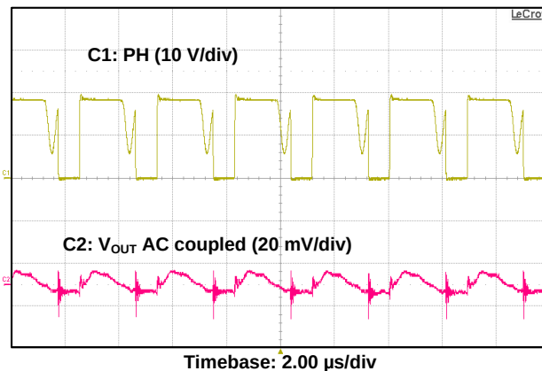
Figure 8. DCM Output Voltage Ripple
