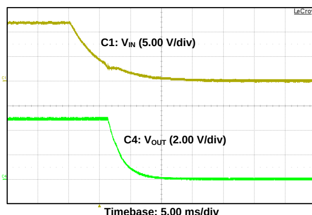
Figure 16. Turn Off With V_{IN}
