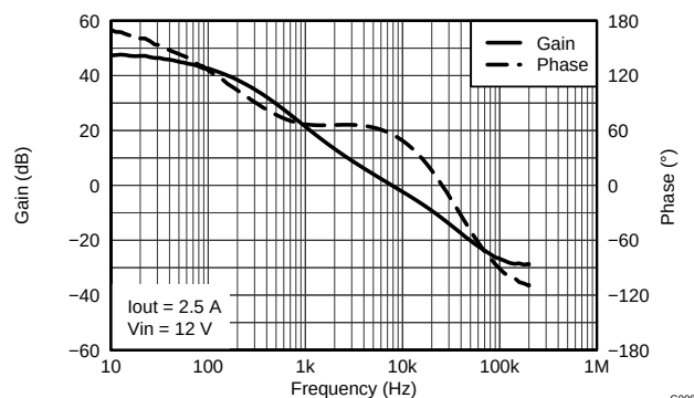
Figure 6. Loop Response
