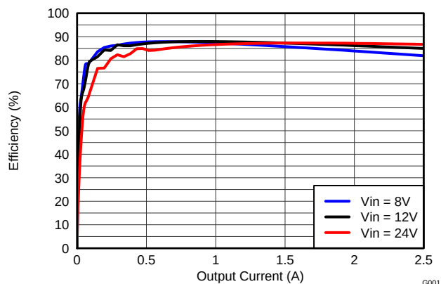
Figure 1. Efficiency
