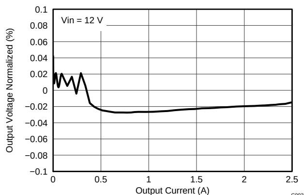
Figure 3. Output Voltage Load Regulation
