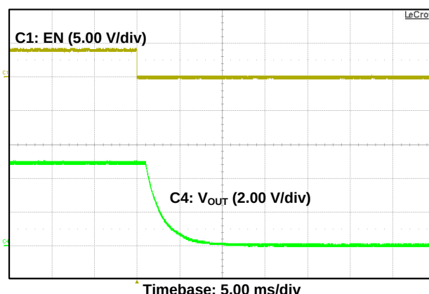
Figure 14. Turn Off With EN
