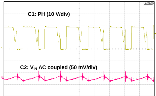
Timebase: 2.00 \mu s/div Figure 11. DCM Input Voltage Ripple
