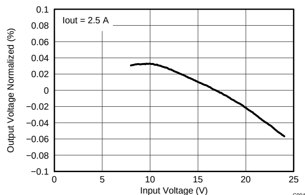
Figure 4. Output Voltage Line Regulation
