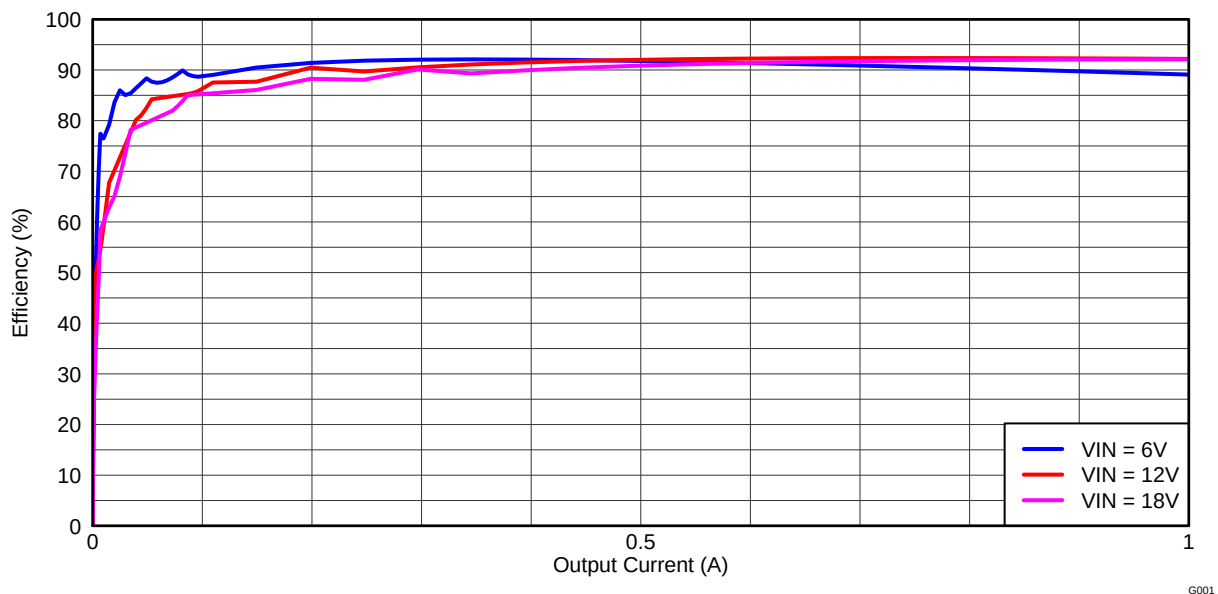
Figure 1. TPS55340EVM-147 Efficiency
