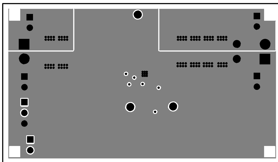
Figure 19. TPS55340EVM-017 Internal Layer-1 Layout
