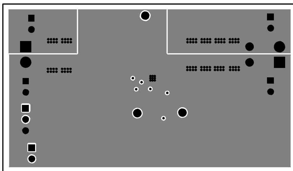
Figure 20. TPS55340EVM-017 Internal Layer-2 Layout
