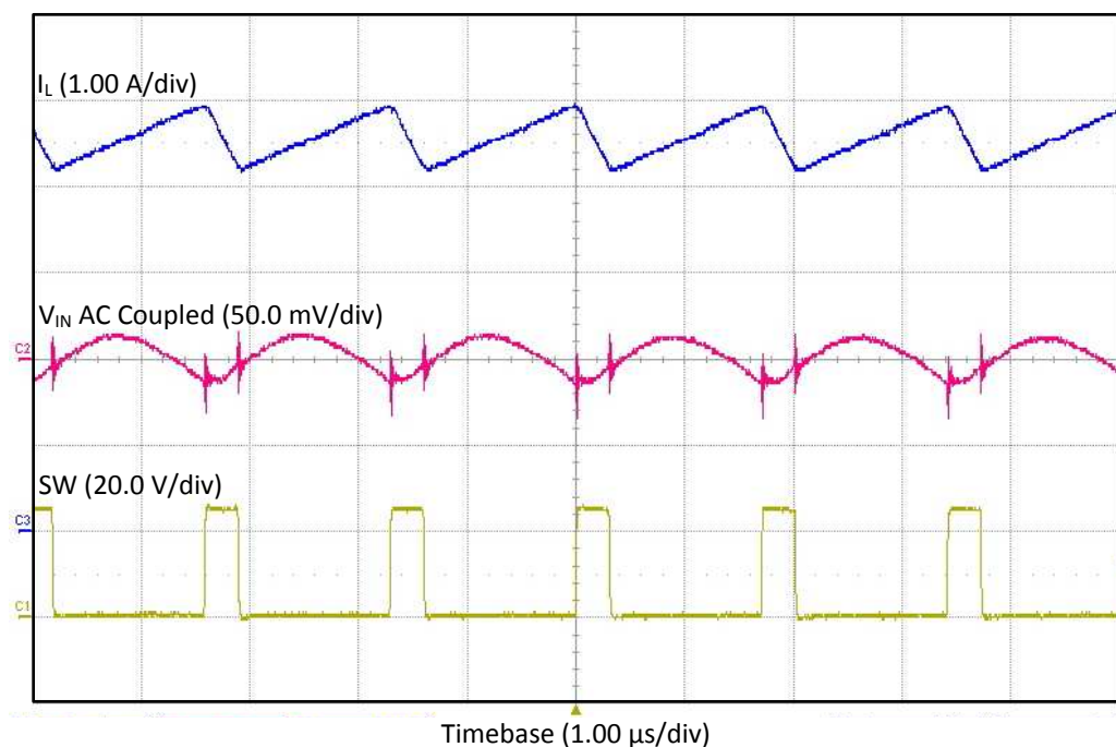
Figure 11. TPS55340EVM-017 V IN = 5-V Input Voltage Ripple
