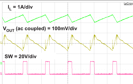
Figure 20. CCM PWM Operation
