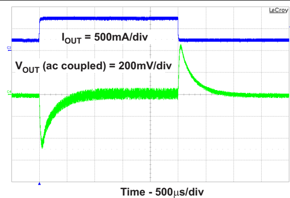
Figure 28. Load Transient Response
