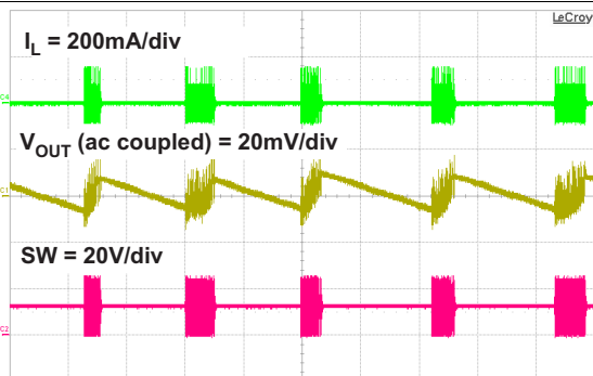
Figure 22. Pulse Skipping
