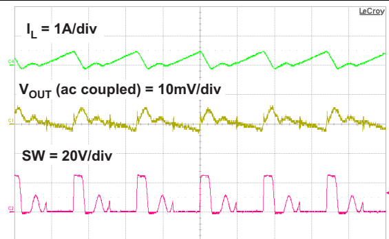
Figure 21. DCM PWM Operation
