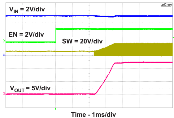
Figure 30. Output Voltage Soft-start
