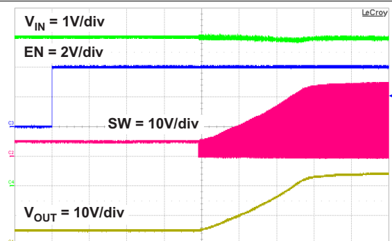
Figure 23. Start-Up
