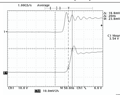
Figure 4. Input Current with Slope Control, SCR1 = 0, SCR0 = 1, Input-Current Slew Rate = 6.25 A/μs, I_L = 500 mA, V_{(driver)} = 15 V
