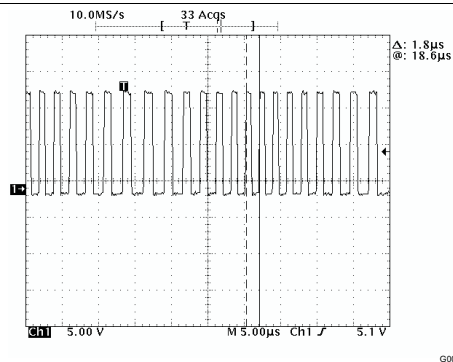
Figure 7. Low-Power-Mode Operation, I_L = 15 \text{ mA} , C_O = 47 \mu\text{F}
