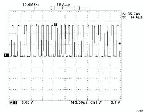
Figure 8. Minimum Switching Frequency (333 kHz) with Modulation Enabled, R_{\text{mod}} = 12 \text{ k}\Omega , I_L = 200 \text{ mA}
