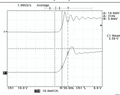
Figure 3. Input Current with Slope Control, SCR0 = 0, SCR1 = 0, Input-Current Slew Rate = 2.8 A/μs, I_L = 500 mA, V_{(driver)} = 15 V
