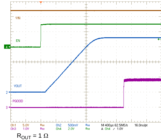
Figure 50. EN Start-up
