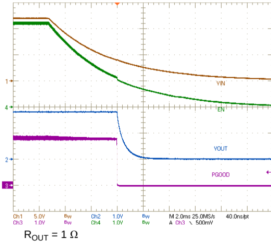
Figure 49. V_{IN} Shutdown
