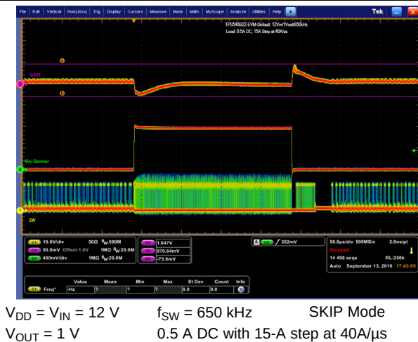
Figure 24. Transient Response Peak-to-Peak
