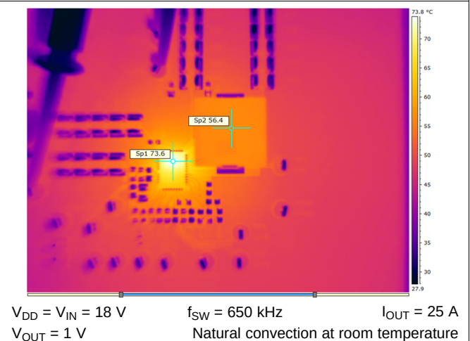
Figure 10. Thermal Image
