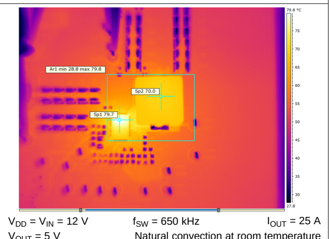
Figure 12. Thermal Image
