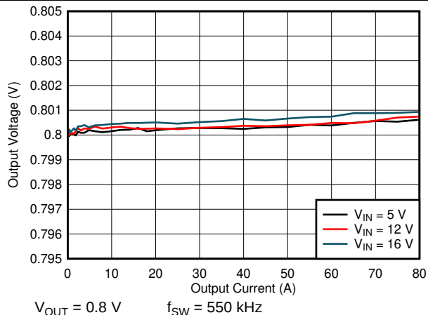
Figure 129. Load Regulation
