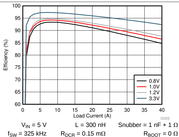
Figure 9. TPS546D24A Efficiency vs Output Current
