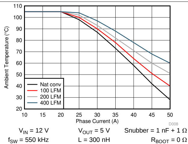
Figure 8. TPS546D24A Safe Operating Area
