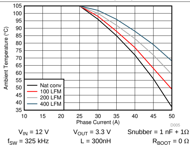
Figure 5. TPS546D24A Safe Operating Area
