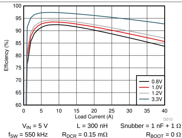
Figure 10. TPS546D24A Efficiency vs Output Current
