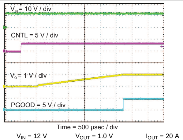
Figure 121. Start-Up from EN/UVLO
