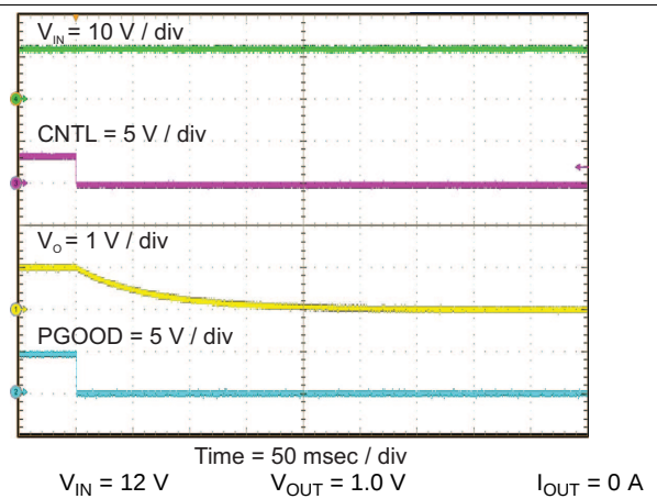
Figure 123. Shutdown from CNTL
