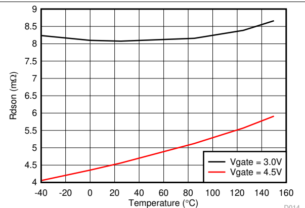
Figure 14. High-Side MOSFET On-Resistance ( R_{DS(on)} ) vs Junction Temperature
