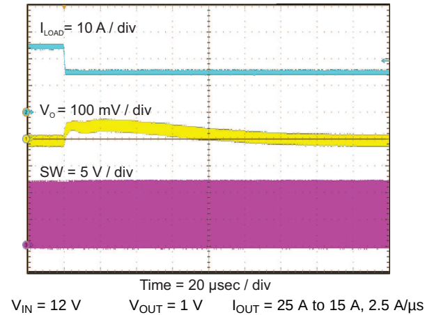
Figure 125. Load Transient Response
