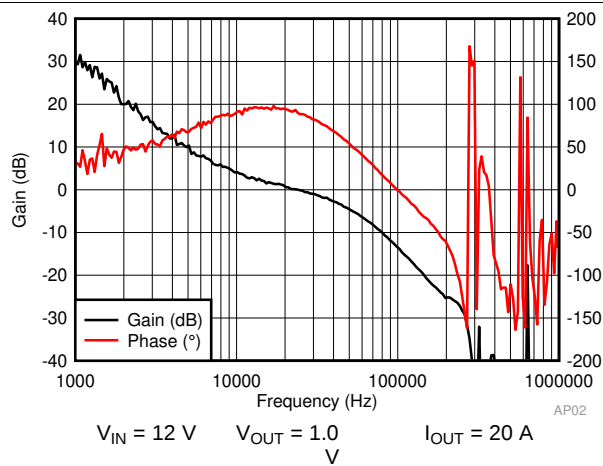
Figure 120. Total-Loop Bode Plot
