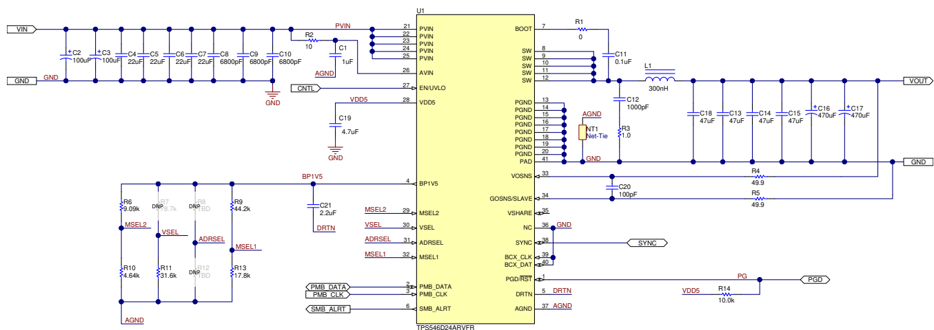
Figure 117. TPS546D24A Stand Alone Application
