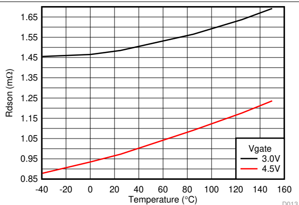
Figure 13. Low-Side MOSFET On-Resistance ( R_{DS(on)} ) vs Junction Temperature
