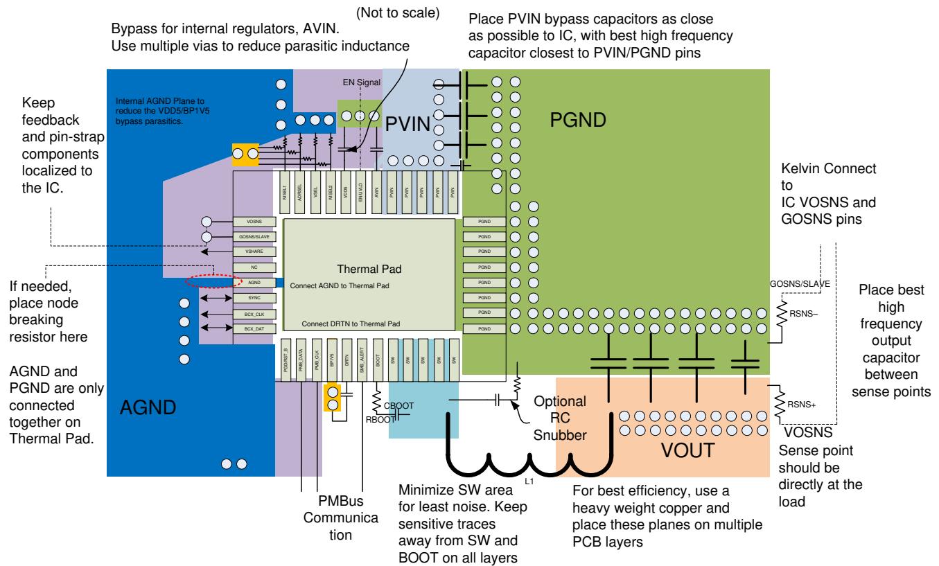
Figure 134. PCB Layout Recommendation
