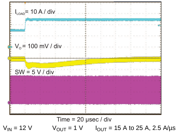
Figure 124. Load Transient Response
