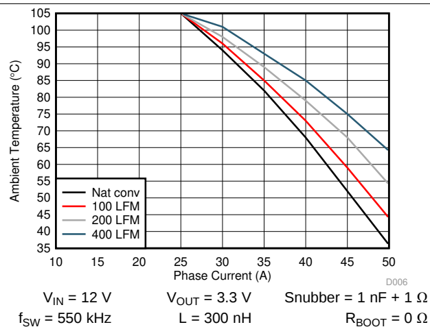
Figure 6. TPS546D24A Safe Operating Area
