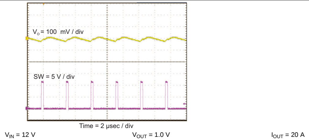
Figure 126. V_{OUT} Steady-State Ripple
