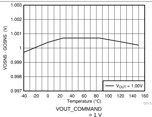
Figure 15. Output Voltage vs Junction Temperature
