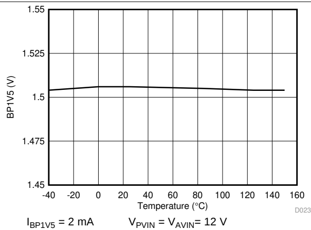
Figure 19. BP1V5 Voltage vs Junction Temperature
