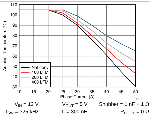
Figure 7. TPS546D24A Safe Operating Area
