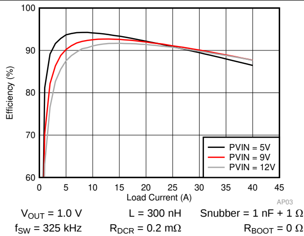
Figure 118. Efficiency vs Output Current
