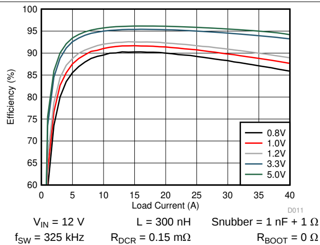
Figure 11. TPS546D24A Efficiency vs Output Current
