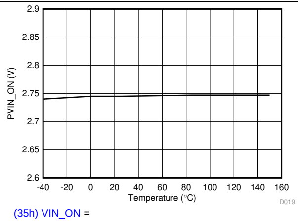
Figure 20. Turnon Voltage vs Junction Temperature
