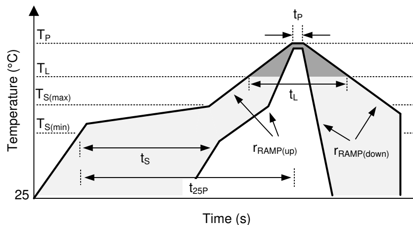
Figure 135. Recommended Reflow-Oven Thermal Profile
