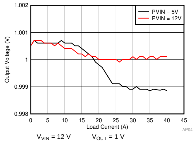
Figure 119. Load Regulation
