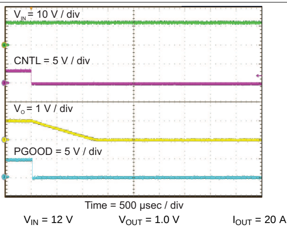
Figure 122. Shutdown from CNTL
