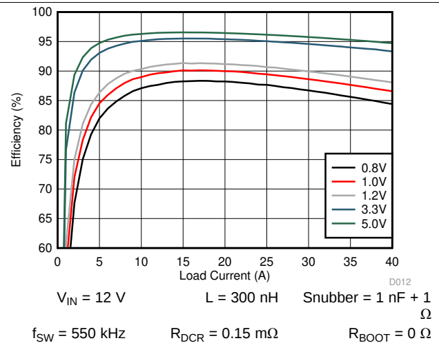
Figure 12. TPS546D24A Efficiency vs Output Current
