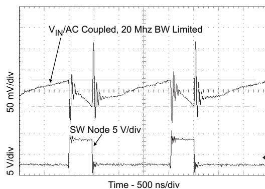
Figure 10. TPS54678EVM-155 Input Ripple at 6 V_{IN} and 6 A
