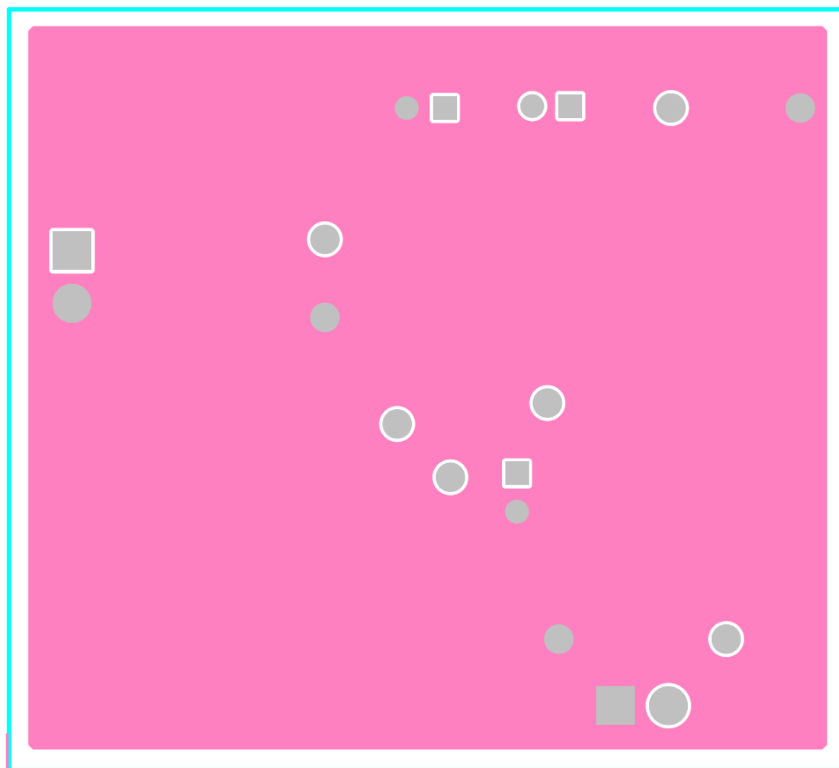
Figure 20. TPS54678EVM-155 Layout 2
