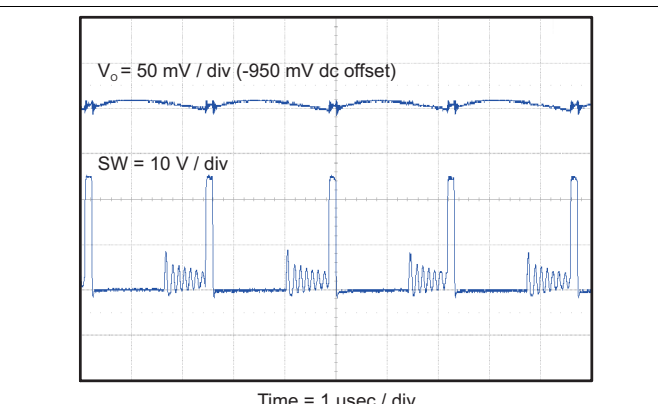
Figure 16. DCM Voltage Ripple at Output
