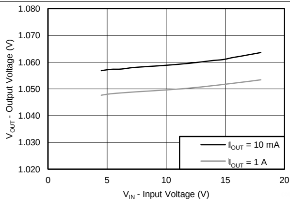
Figure 6. 1.05-V Output Voltage vs Input Voltage
