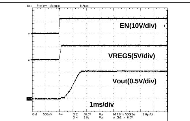
Figure 14. Start-Up Waveform
