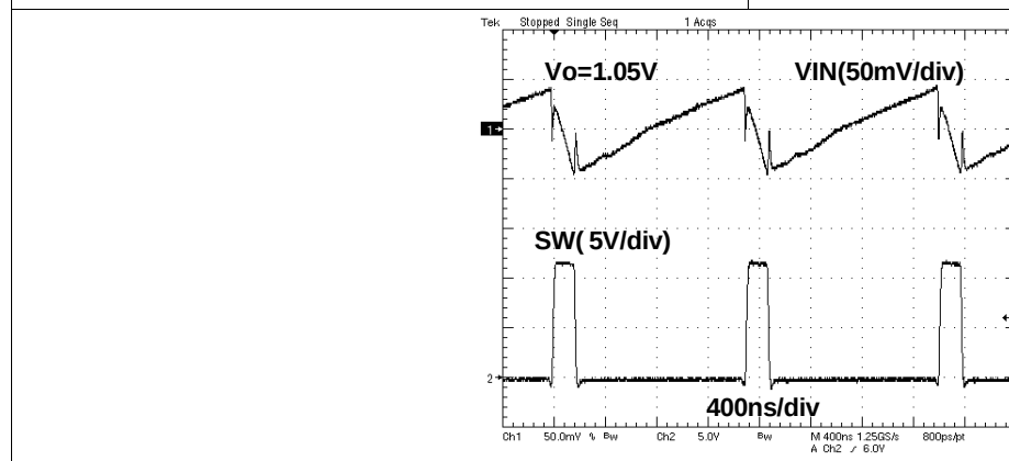
Figure 17. Voltage Ripple at Input
