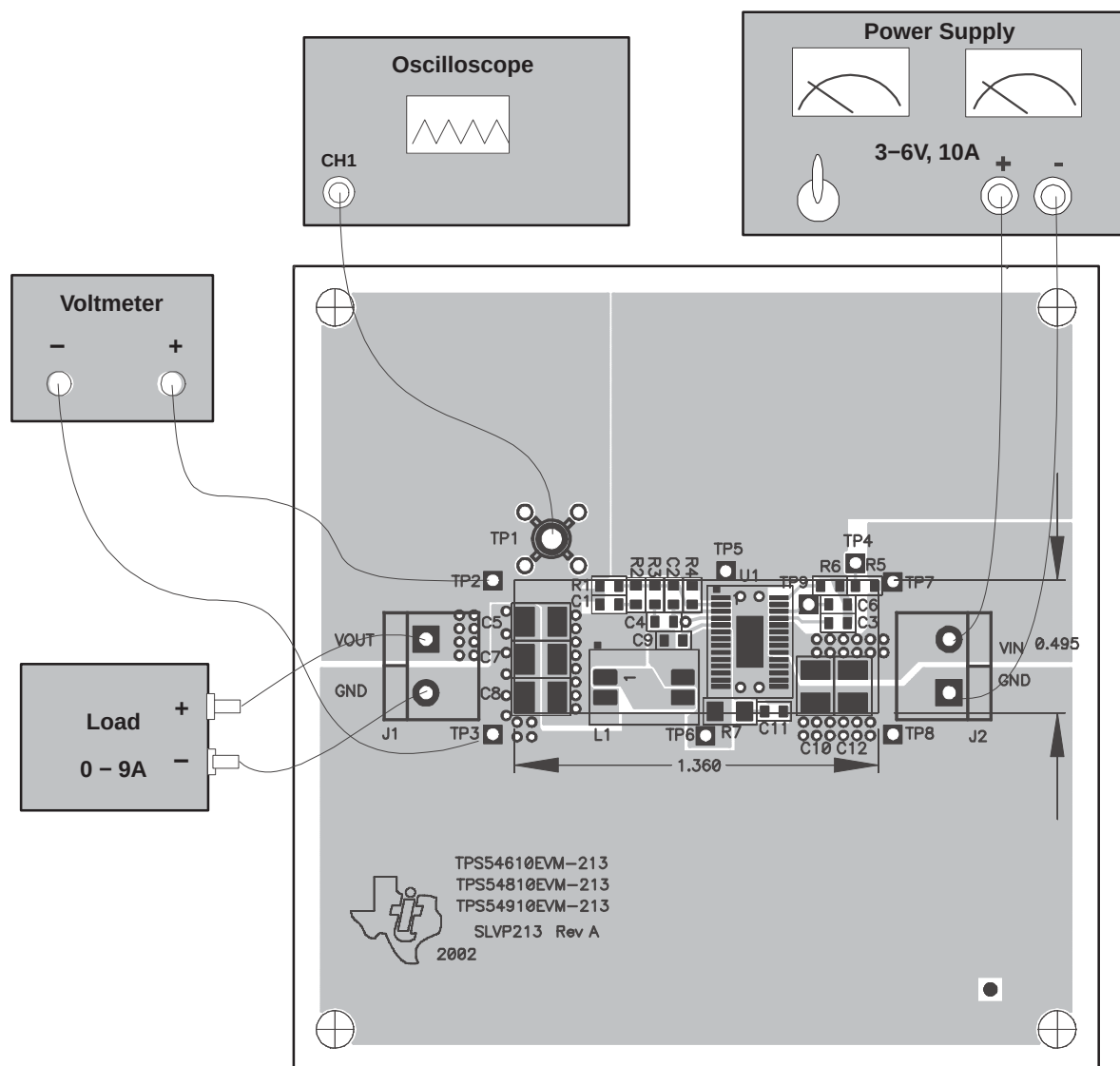
Figure 2–1. Connection Diagram
