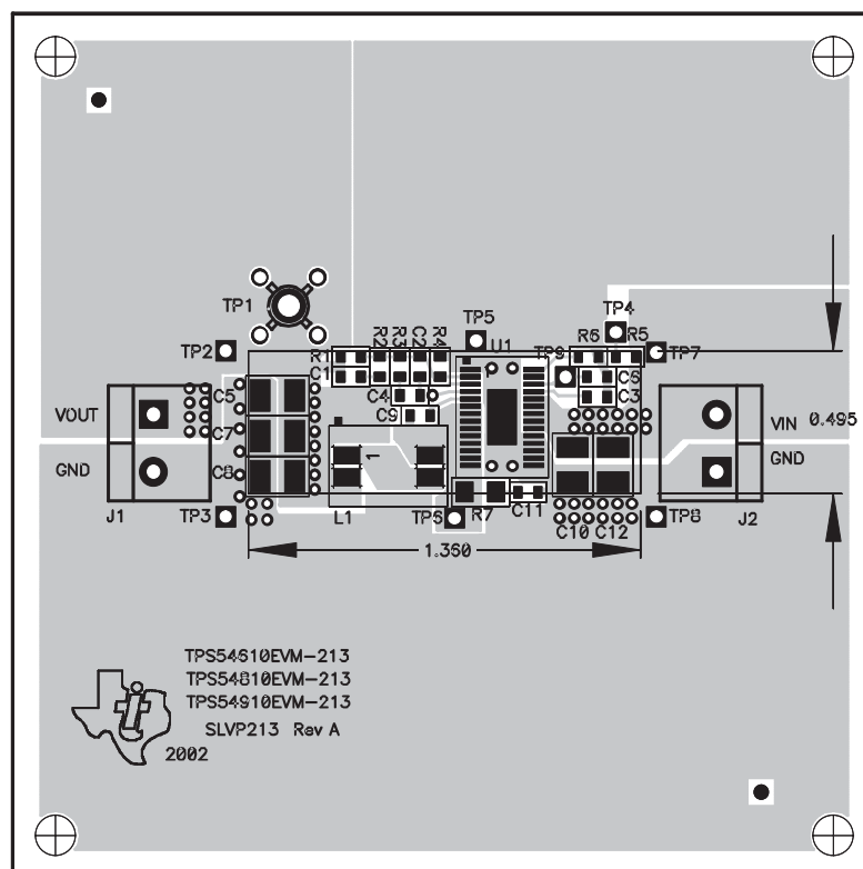
Figure 3–5. Top-Side Assembly
