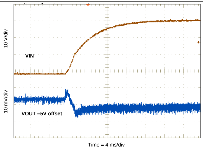
Figure 52. Line Transient (8 V to 40 V)
