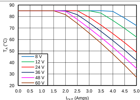
Figure 48. 5-V Output with 400-kHz Switching Frequency
