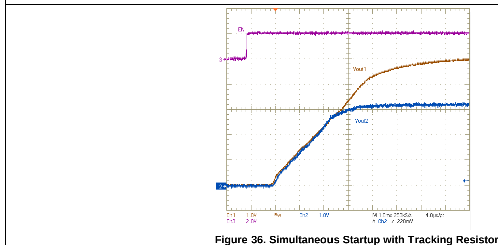
Figure 36. Simultaneous Startup with Tracking Resistor
