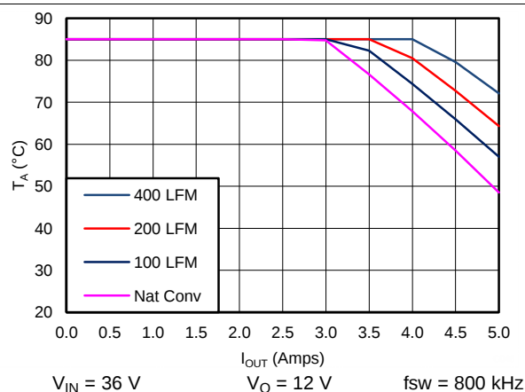
Figure 50. Air Flow Conditions
