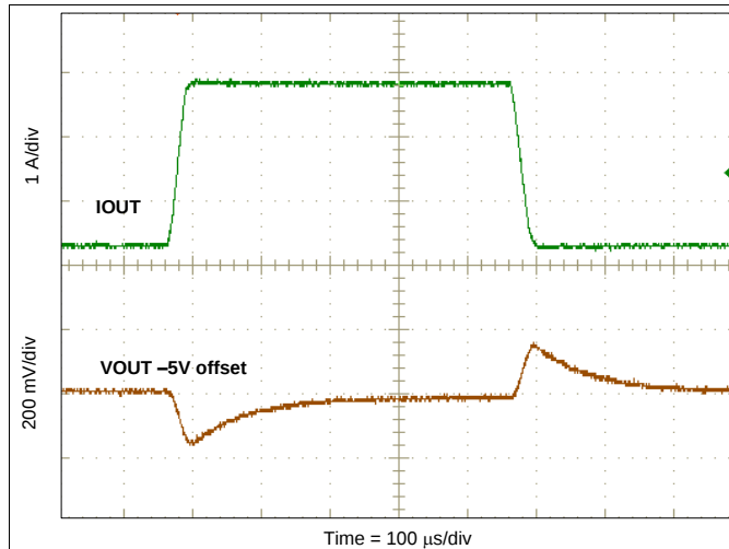
Figure 51. Load Transient
