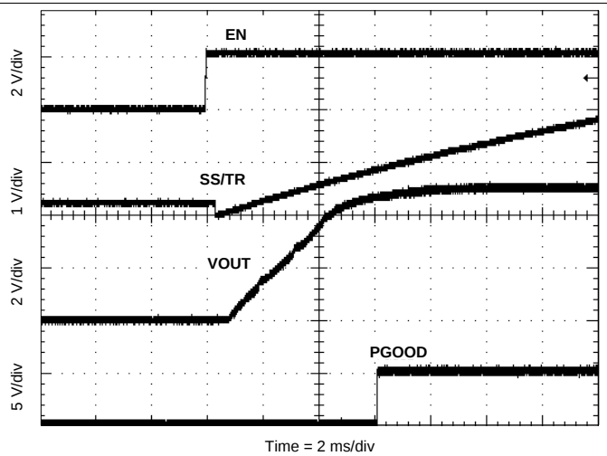
Figure 54. Start-up With EN
