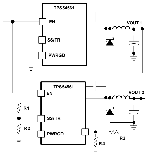
Figure 33. Schematic for Ratio-Metric and Simultaneous Start-Up Sequence
