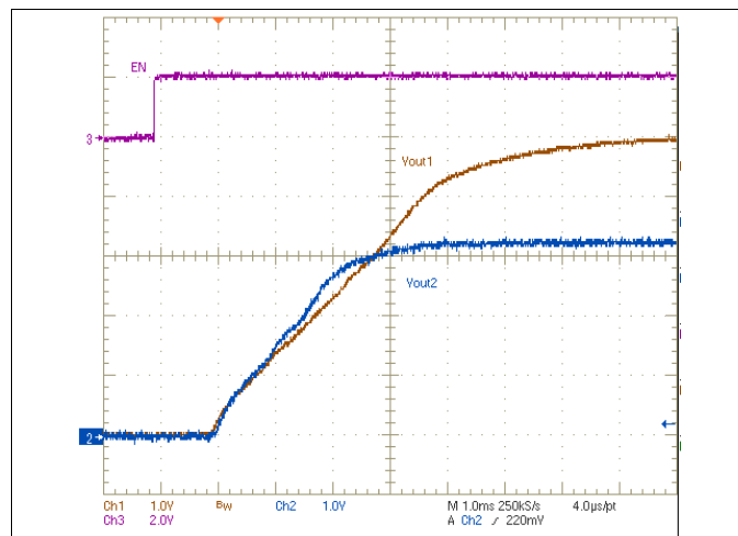
Figure 34. Ratio-Metric Startup with Tracking Resistors
