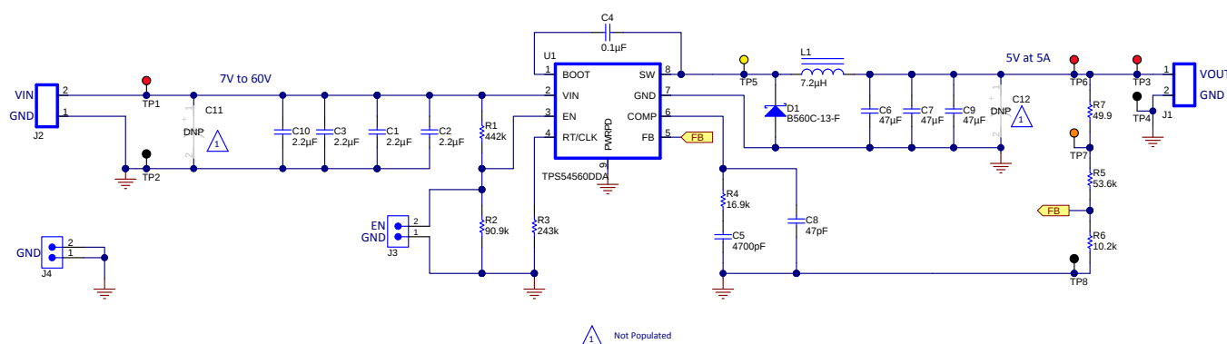
Figure 2. TPS54560EVM-515 Schematic
