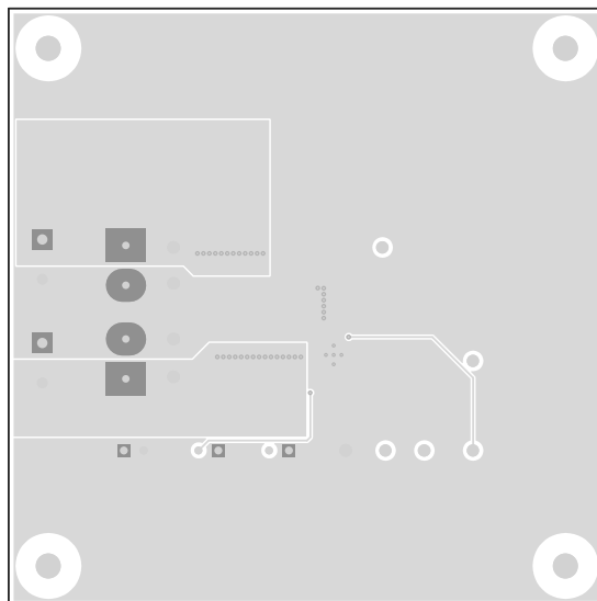
Figure 25. TPS54541EVM-555 Bottom-Side Layout
