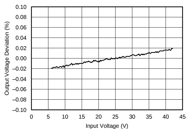
Figure 6. Regulation Versus Input Voltage
