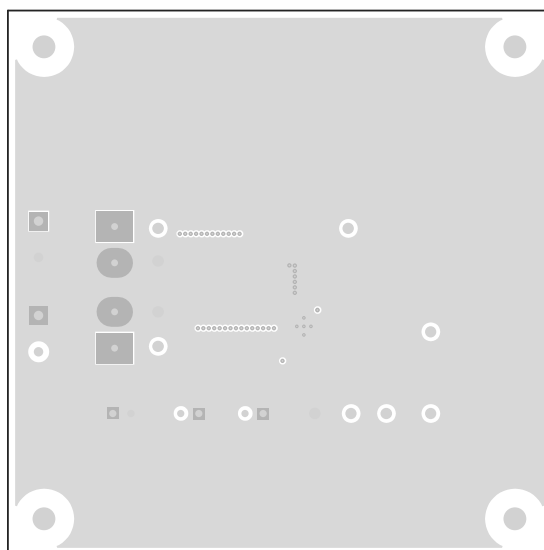
Figure 24. TPS54541EVM-555 Layer 3 Layout
