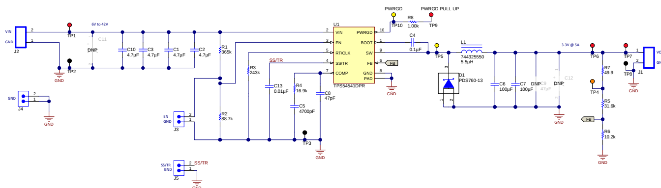
Figure 2. TPS54541EVM-555 Schematic
