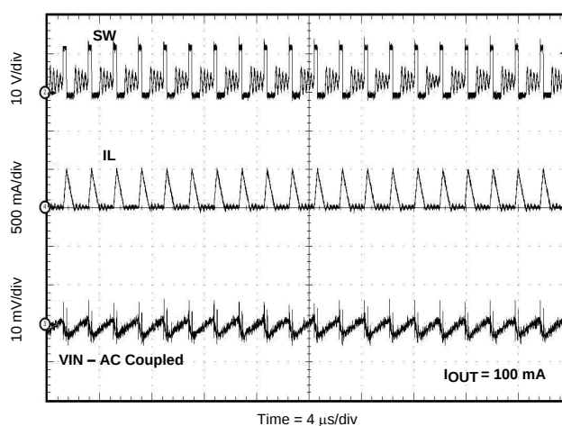
Figure 11. Input Voltage Ripple DCM
