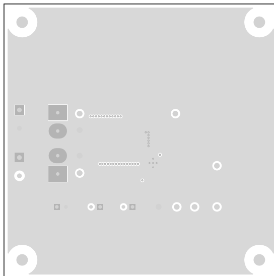
Figure 23. TPS54541EVM-555 Layer 2 Layout
