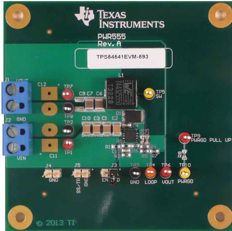
Figure 1. TPS54541EVM-555 Board
