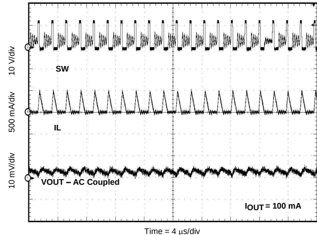
Figure 56. Output Ripple DCM
