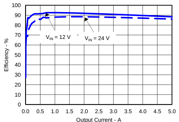
TPS54531 Efficiency
