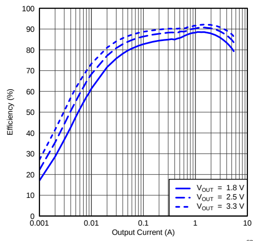
Figure 11. Light Load Efficiency vs Output Current
