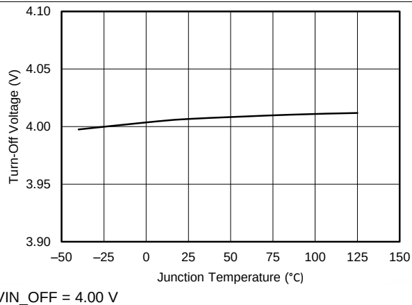
Figure 9. Turn-Off Voltage vs. Junction Temperature
