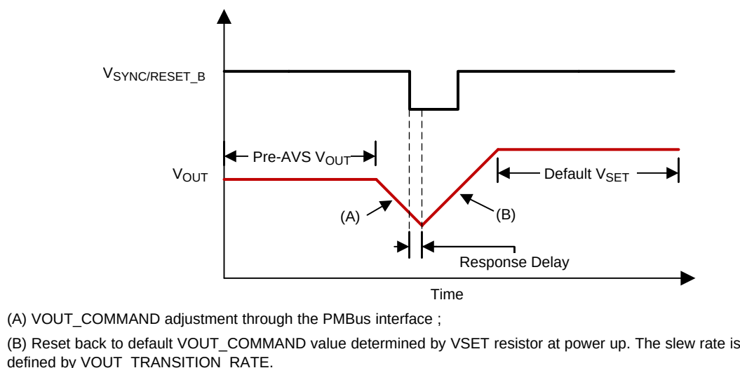
Figure 35. Output Voltage Reset
