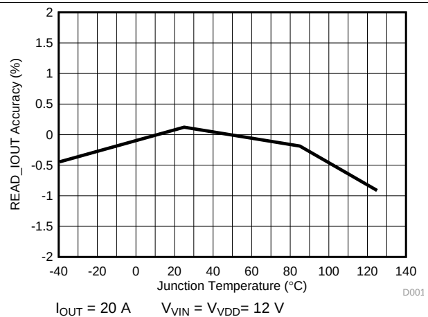
Figure 14. READ_IOUT Accuracy vs. Junction Temperature
