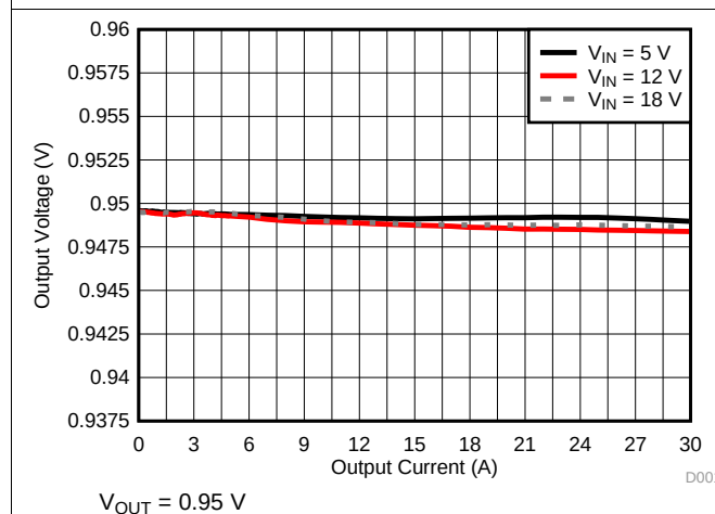
Figure 47. Load Regulation
