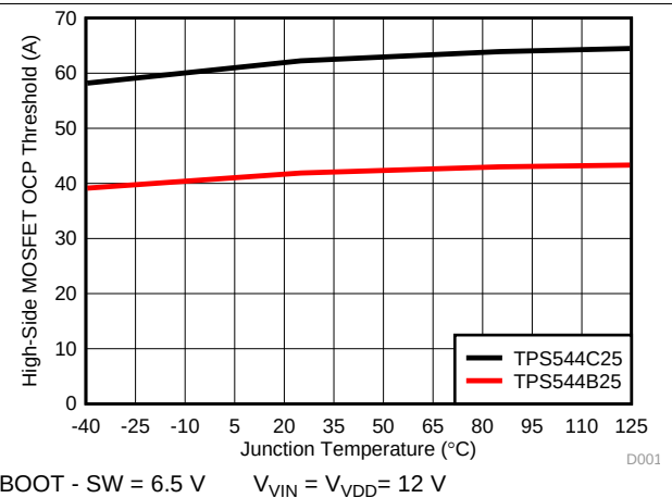
Figure 16. High-Side Overcurrent Protection vs. Junction Temperature
