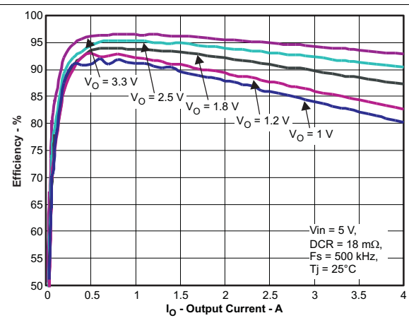
Figure 20. Efficiency vs Load Current
