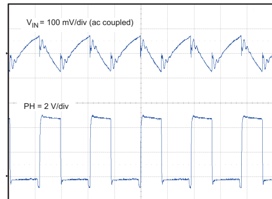
Figure 47. Input Ripple, I_{OUT} = 4 A
