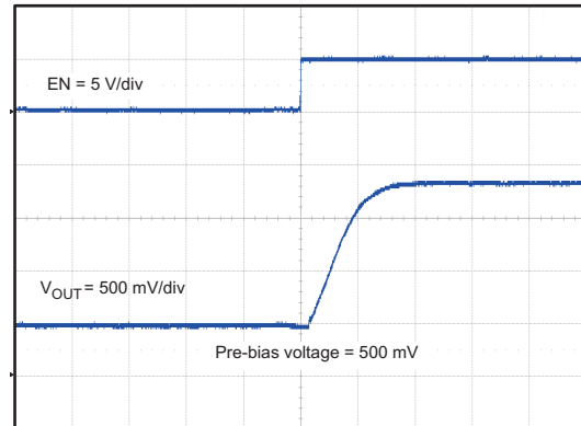
Figure 43. Power Up into Prebias Voltage
