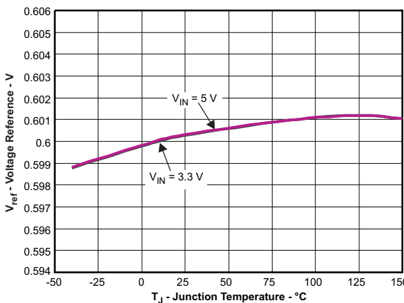
Figure 5. Voltage Reference vs Temperature
