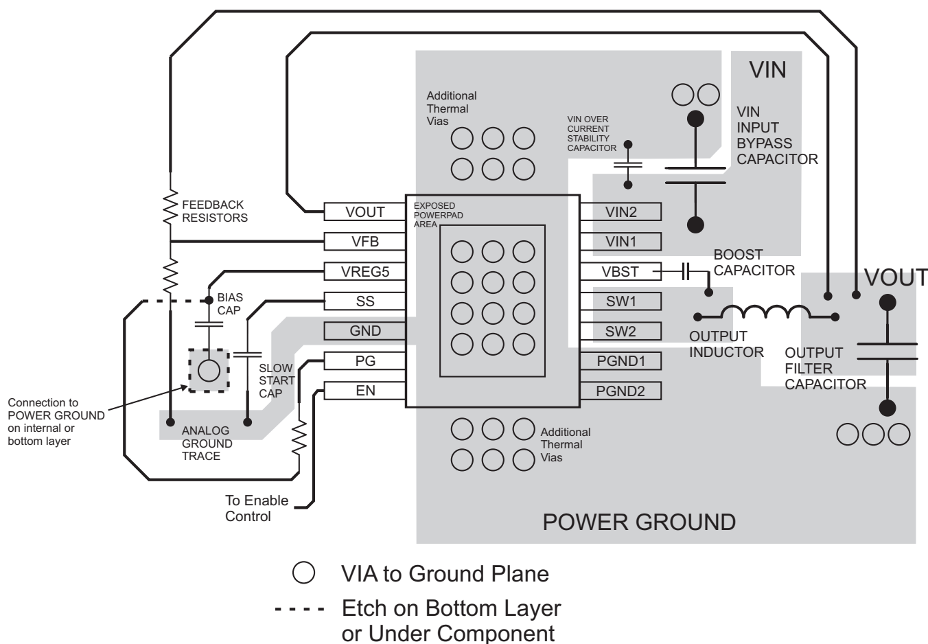
Figure 16. PCB Layout
