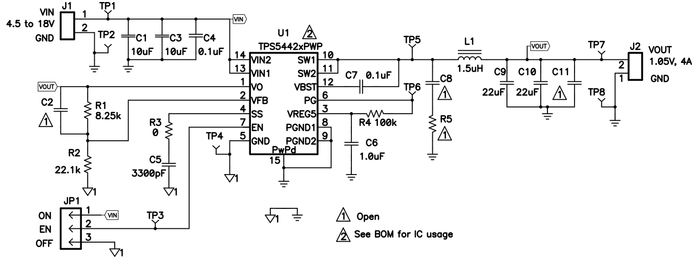
Figure 16. TPS54425EVM-608 Schematic Diagram
