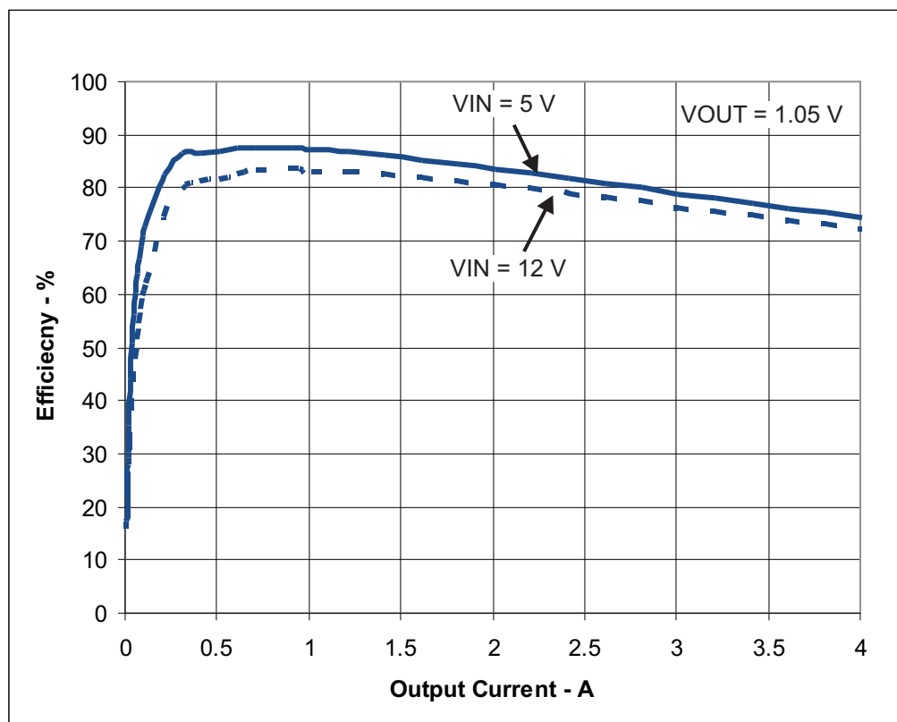
Figure 1. TPS54425EVM-608 Efficiency
