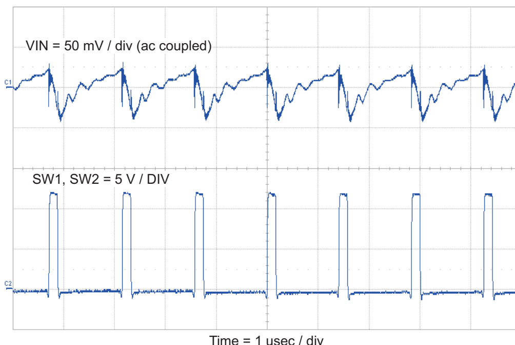
Figure 7. TPS54425EVM-608 Input Voltage Ripple
