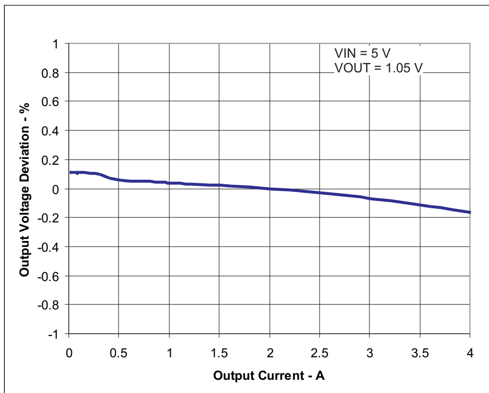
Figure 3. TPS54425EVM-608 Load Regulation
