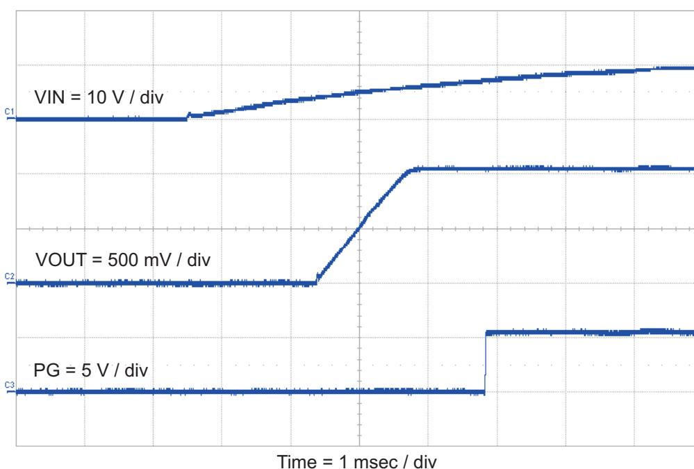
Figure 8. TPS54425EVM-608 Start-Up Relative to V_{IN}
