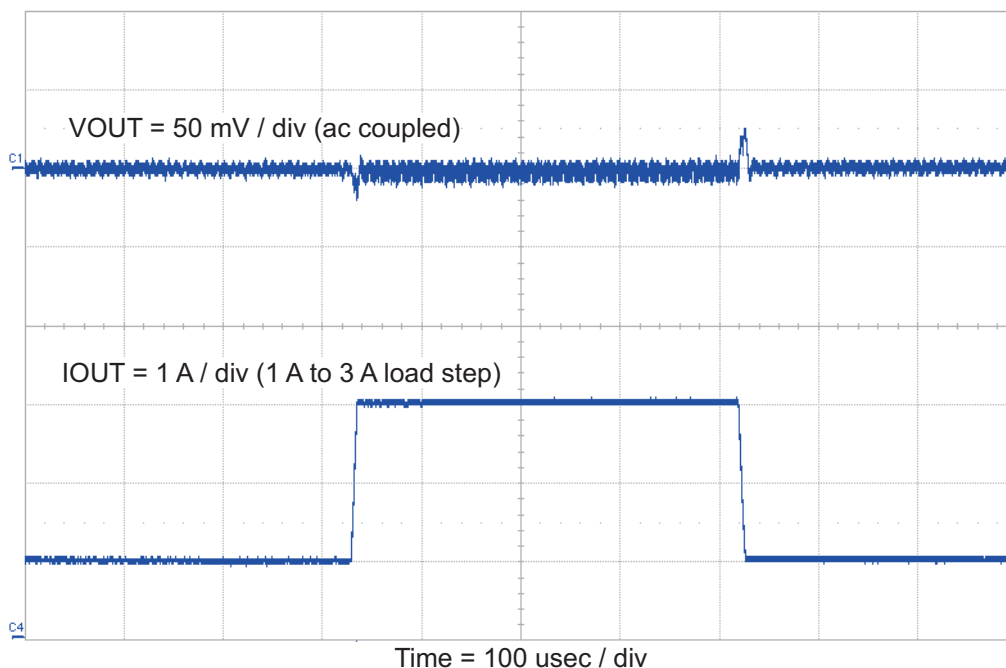
Figure 5. TPS54425EVM-608 Load Transient Response
