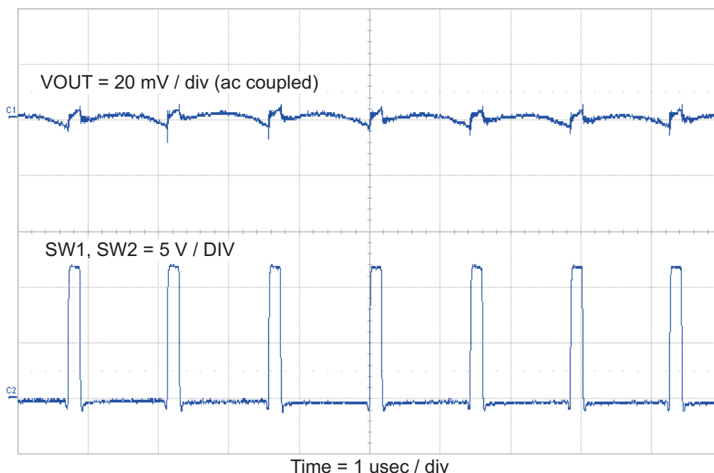
Figure 6. TPS54425EVM-608 Output Voltage Ripple
