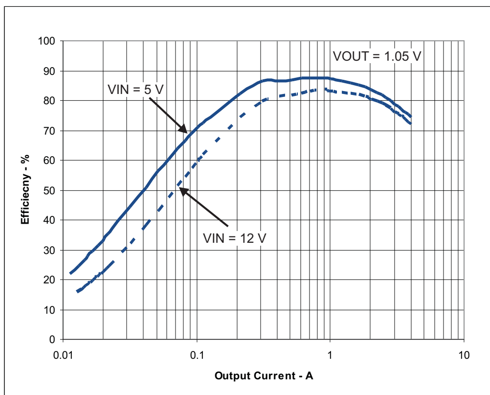
Figure 2. TPS54425EVM-608 Light Load Efficiency
