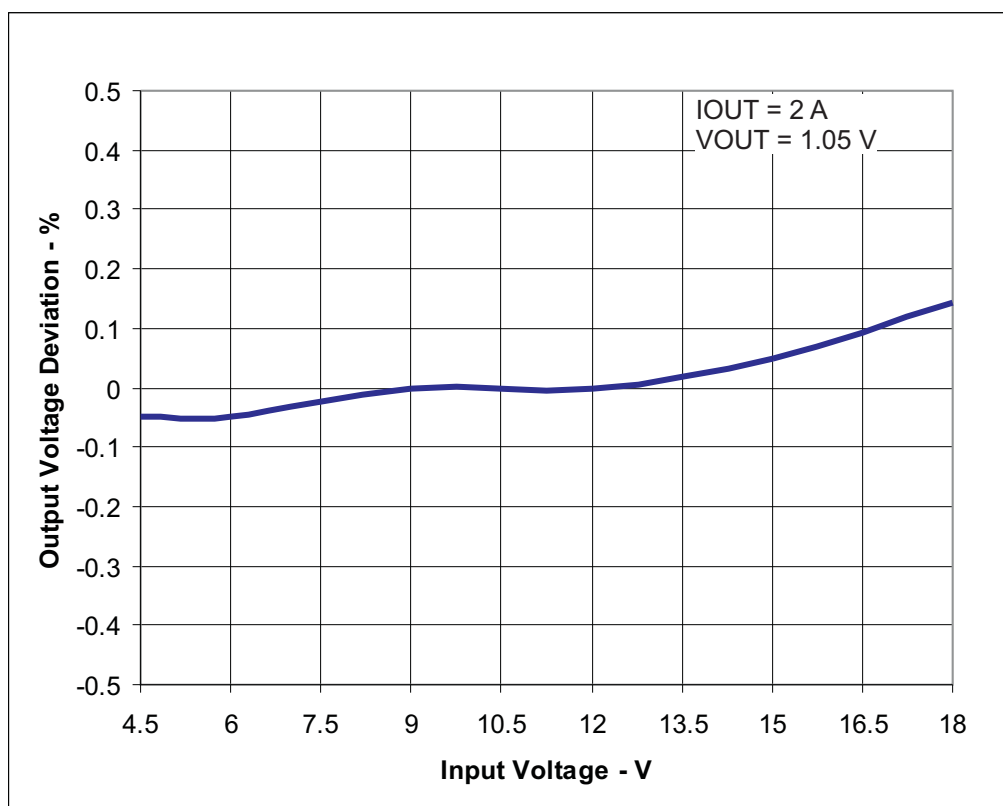
Figure 4. TPS54425EVM-608 Line Regulation
