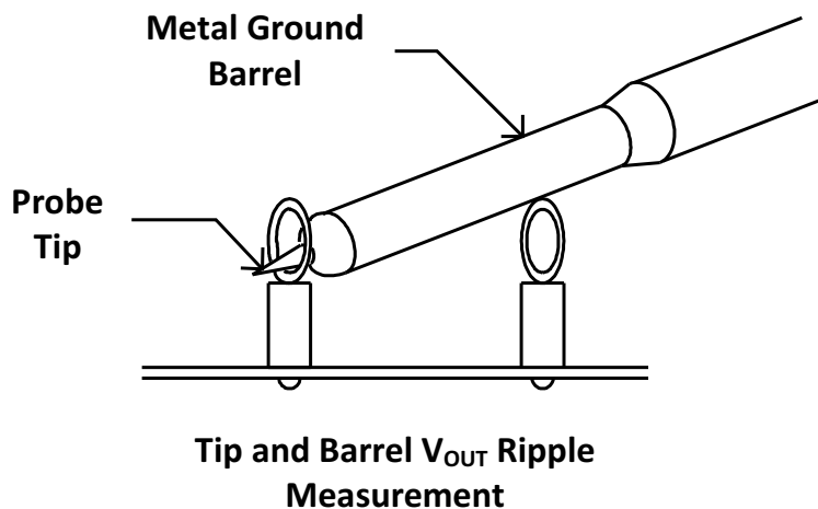
Figure 3. Tip and Barrel Measurement
