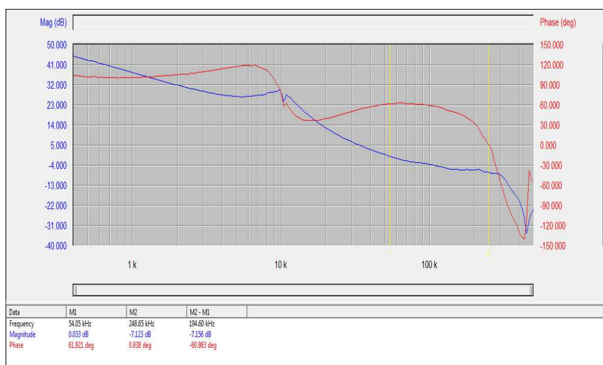
Figure 15. Bode Plot at 0.95- V Output at 12 V_{IN} , 20-A Output
