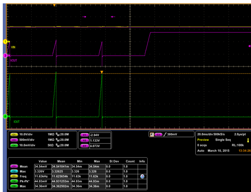
Figure 14. Restart from Overcurrent Protection, 0.95- V Output at 12 V_{IN}
