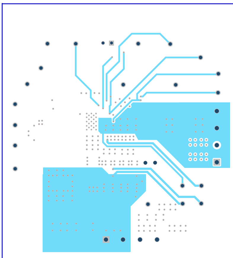
Figure 18. BSR054EVM Inner Layer 2 (Top View)
