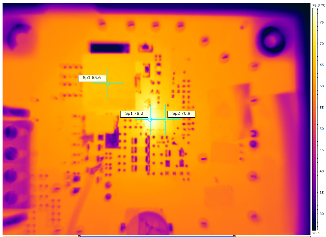
Figure 13. Thermal Image at 0.9-V Output at 12 V IN , 40-A Output, at 25°C Ambient
