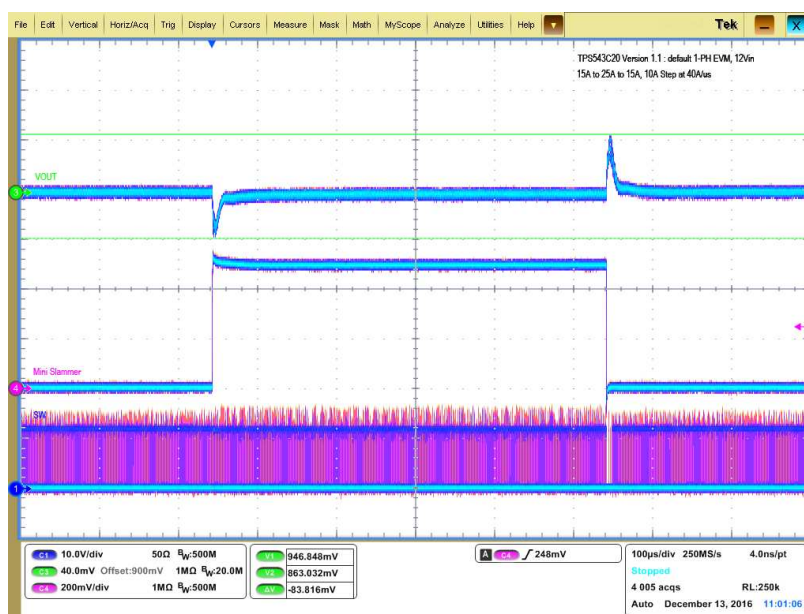
Figure 7. Transient Response of 0.9-V Output at 12- V_{IN} , Transient is 15 A to 25 A to 15 A, the Step is 10 A at 40 A/ \mu s
