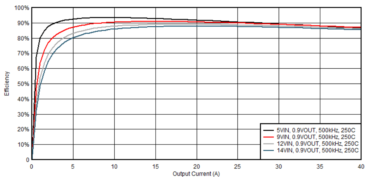
Figure 4. Efficiency of 0.9-V Output vs Load
