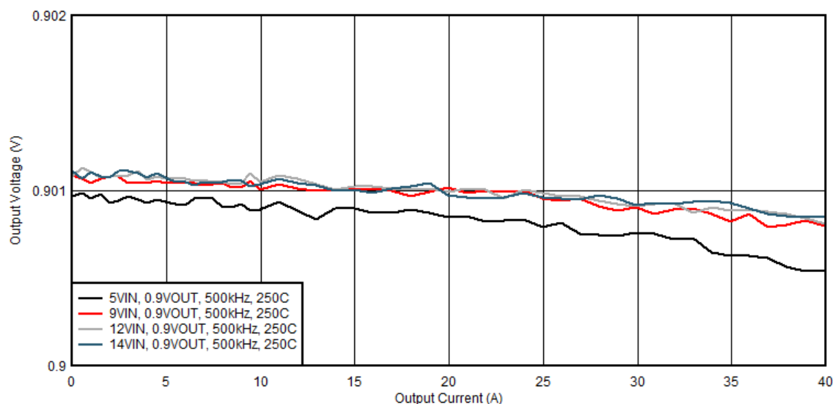
Figure 6. Load Regulation of 0.9-V Output
