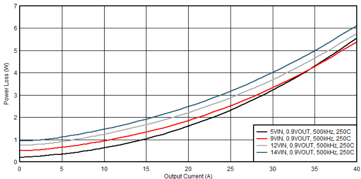
Figure 5. Power Loss of 0.9-V Output vs Load
