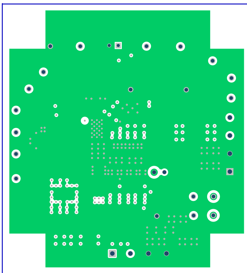
Figure 19. BSR054EVM Inner Layer 3 (Top View)
