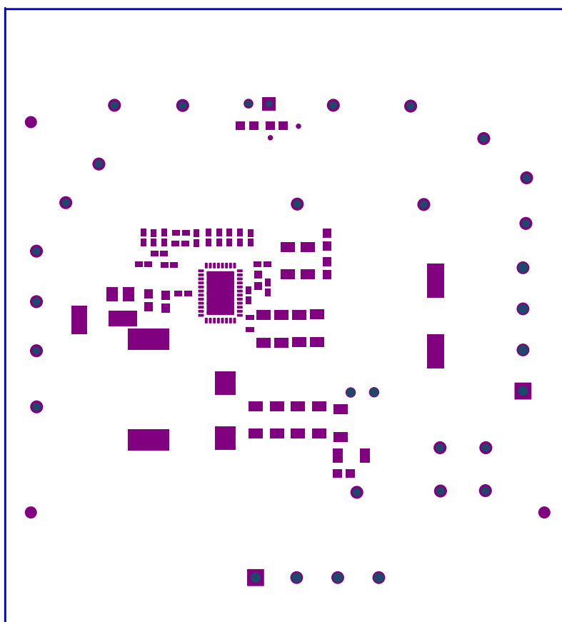
Figure 15. BSR054EVM Top Solder Mask (Top View)
