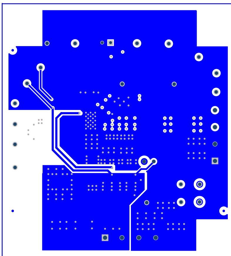
Figure 21. BSR054EVM Bottom Layer (Top View)
