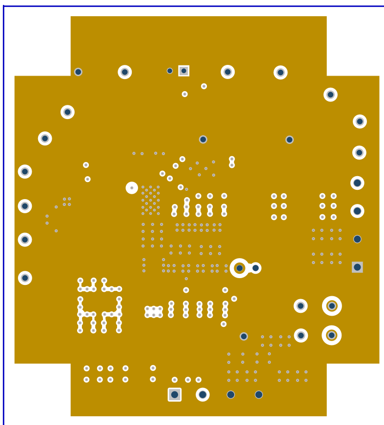
Figure 17. BSR054EVM Inner Layer 1 (Top View)
