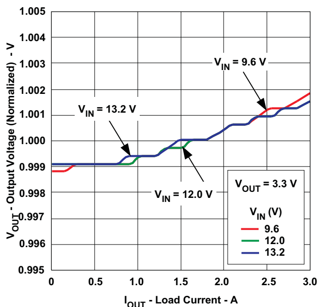
Figure 44. 3.3-V Output Voltage vs. Load Current
