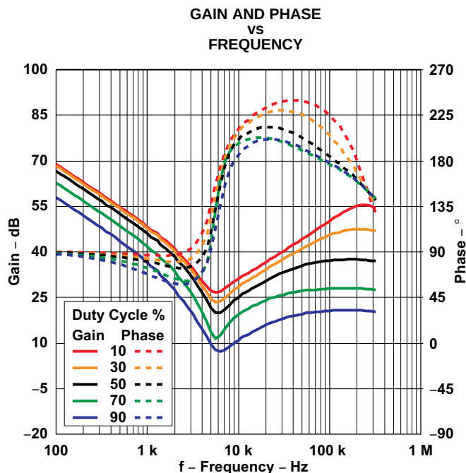
Figure 27. TPS54386 at 200-mA App Ripple Current
