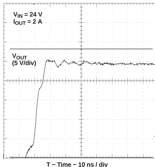
Figure 48. Switch Node Ringing With Snubber and Boost Resistor
