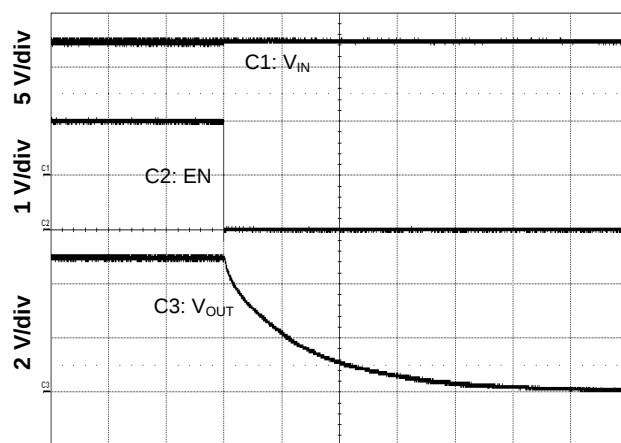
Figure 19. Shutdown Relative to EN
