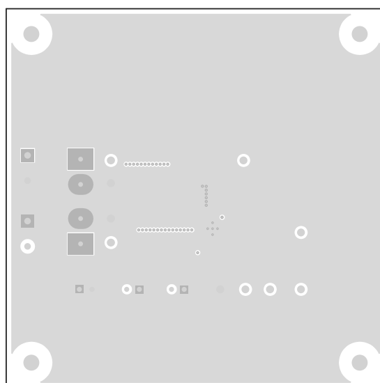
Figure 24. TPS54361EVM-555 Layer 3 Layout
