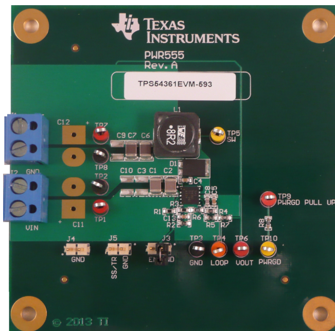
Figure 1. TPS54361EVM-555 Board
