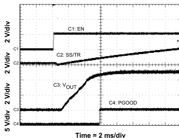
Figure 16. Start Up Relative to EN
