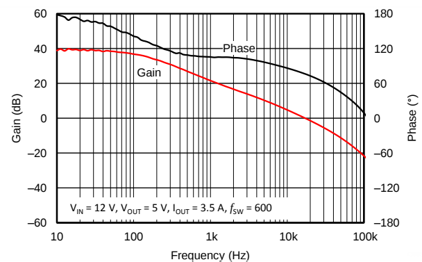
Figure 8. Loop Response
