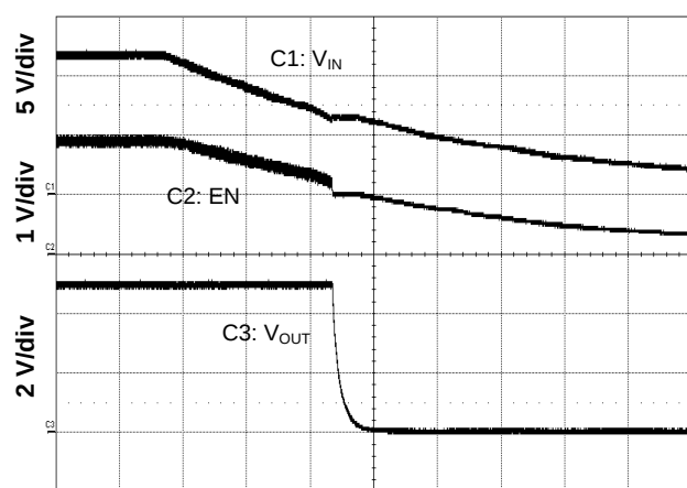
Figure 18. Shutdown Relative to V_{IN}
