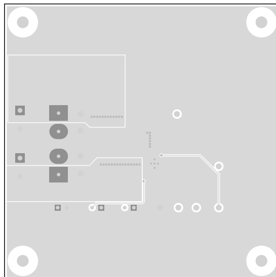
Figure 25. TPS54361EVM-555 Bottom-Side Layout
