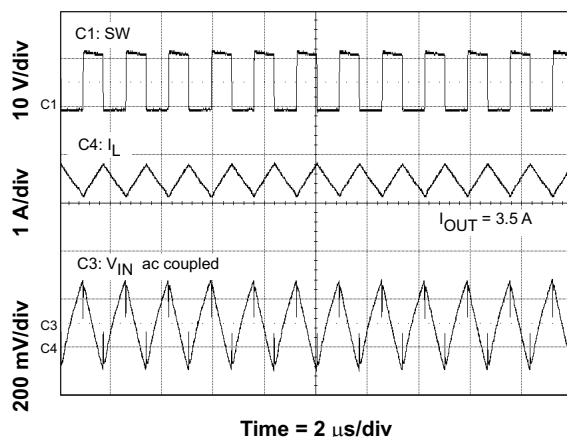
Figure 10. Input Voltage Ripple CCM
