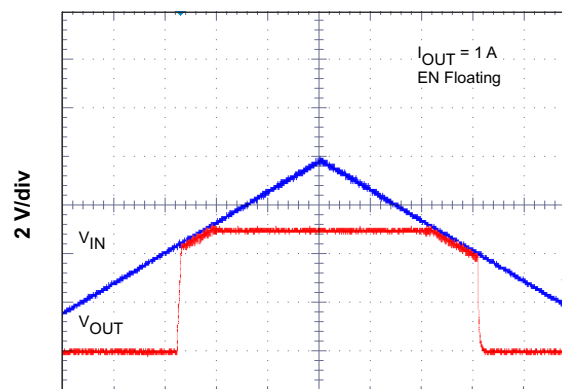
Figure 21. Low Dropout Start Up and Shutdown
