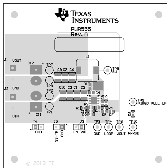
Figure 22. TPS54361EVM-555 Top Assembly and Silkscreen
