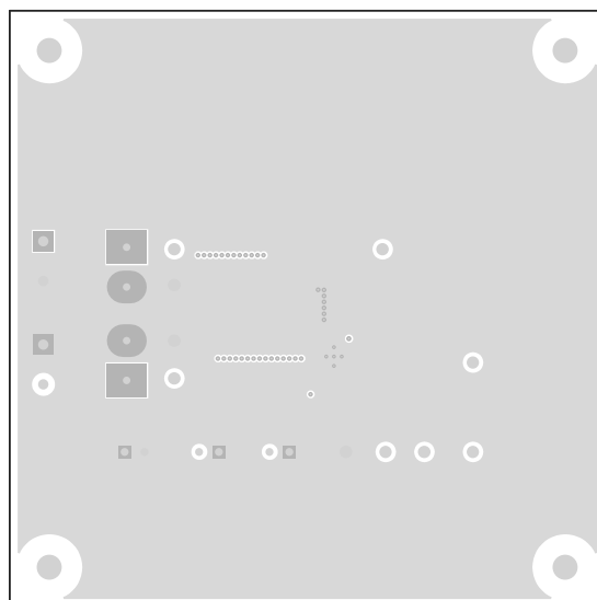
Figure 23. TPS54361EVM-555 Layer 2 Layout
