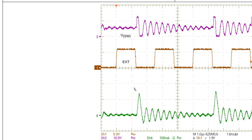
Figure 41. Plot of Synchronizing in Eco-mode
