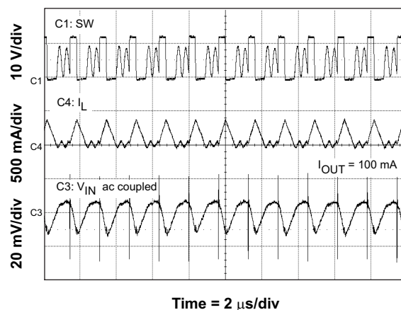
Figure 14. Input Voltage Ripple DCM
