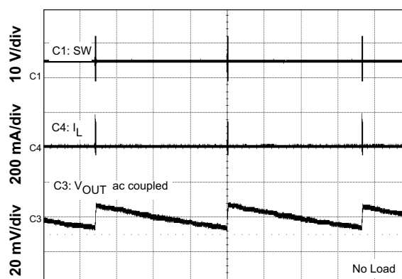
Figure 12. Output Voltage Ripple Eco-mode
