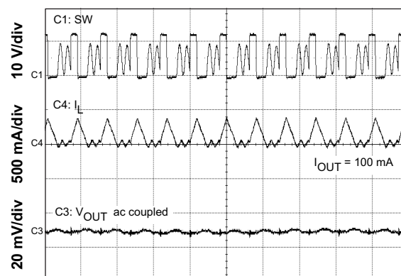
Figure 11. Output Voltage Ripple DCM
