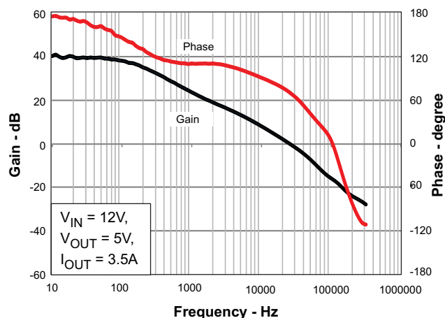
Figure 8. Loop Response
