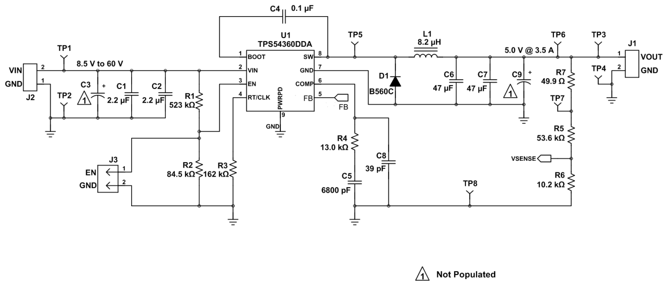
Figure 27. TPS54360EVM-182 Schematic
