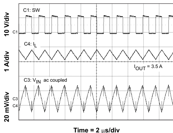
Figure 13. Input Voltage Ripple CCM
