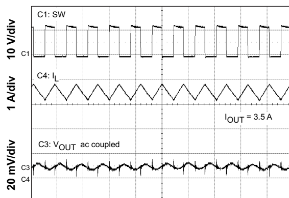
Figure 10. Output Voltage Ripple CCM
