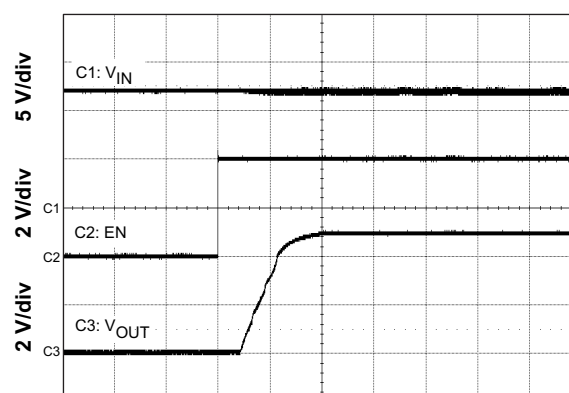
Time = 2 ms/div Figure 16. Start Up Relative to EN
