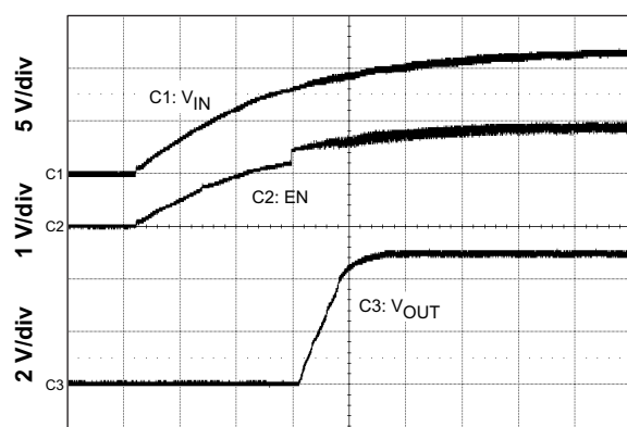
Time = 2 ms/div Figure 15. Start Up Relative to V_{IN}
