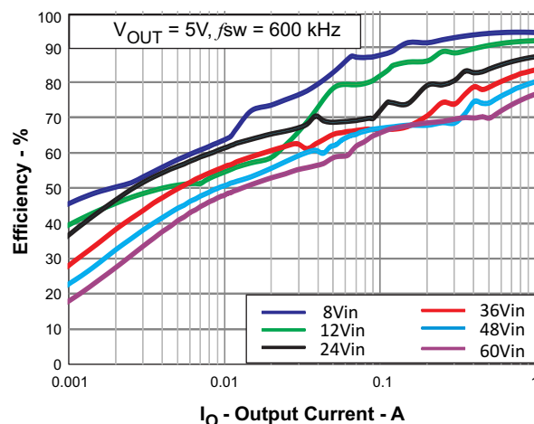
Figure 2. Light-Load Efficiency
