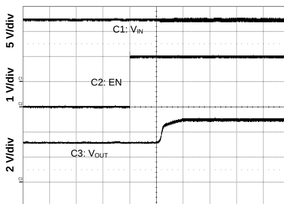
Time = 2 ms/div Figure 17. Prebias Start Up Relative to EN
