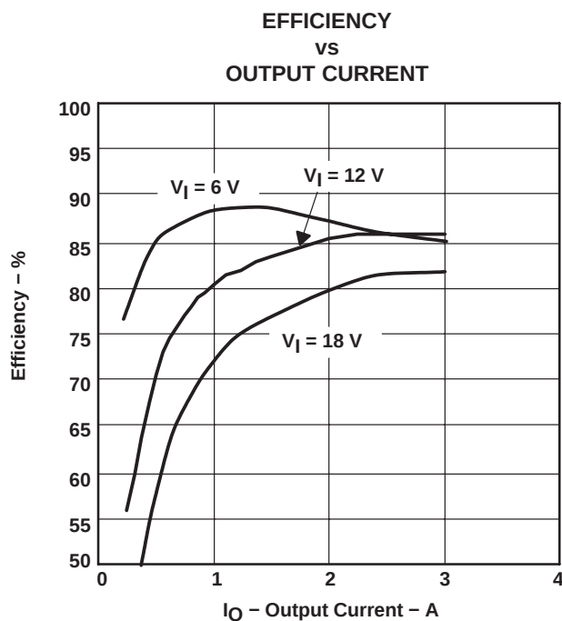
Figure 2-2. Measured Efficiency, TPS54350
