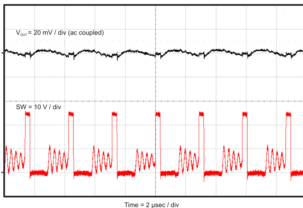
Figure 8. TPS54336EVM-556 Output Ripple, I_{OUT} = 100 \text{ mA}
