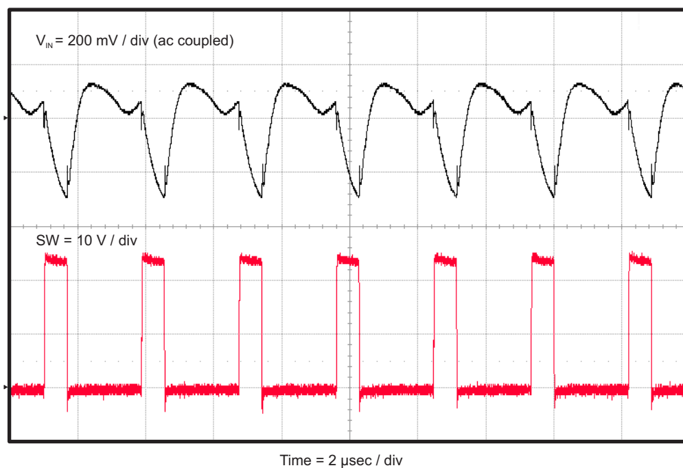
Figure 10. TPS54335EVM-556 Input Ripple
