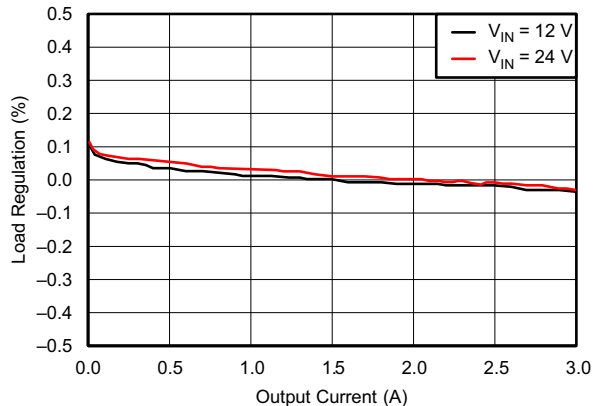
Figure 42. TPS54336A DRC Load Regulation
