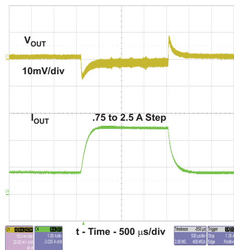
Figure 17. TPS54332 Transient Response
