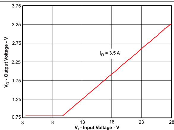
Figure 9. Typical Minimum Output Voltage vs Input Voltage
