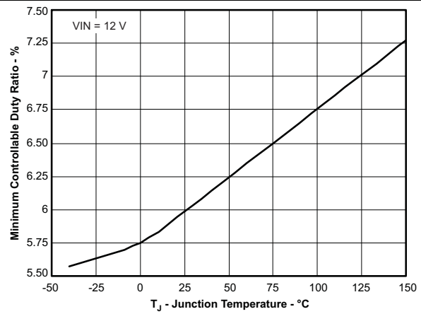
Figure 6. Minimum Controllable Duty Ratio vs Junction Temperature
