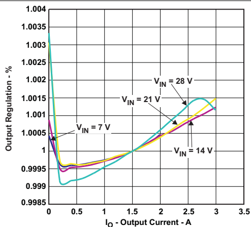
TPS54331 (D Package)
