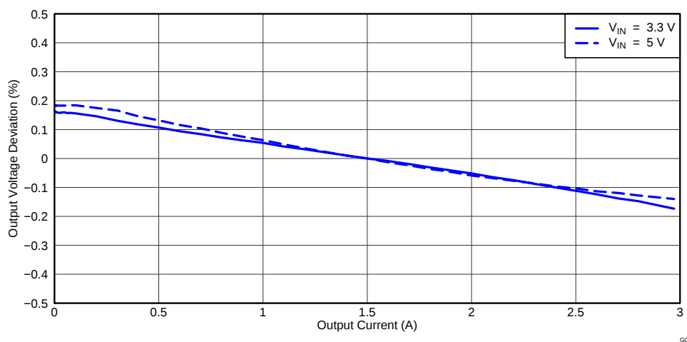
Figure 3. TPS5432EVM-116 Load Regulation
