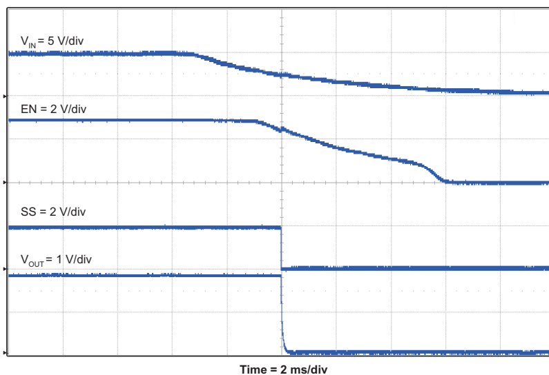
Figure 11. TPS5432EVM-116 Shut Down Relative to V_{IN}
