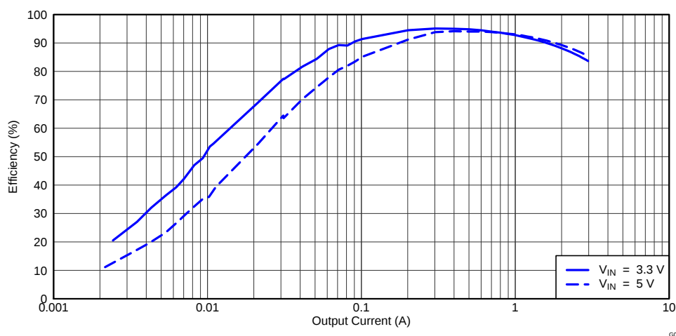
Figure 2. TPS5432EVM-116 Low Current Efficiency
