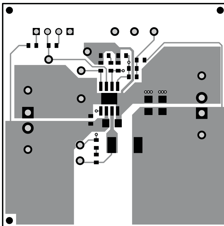
Figure 14. TPS5432EVM-116 Top-Side Layout
