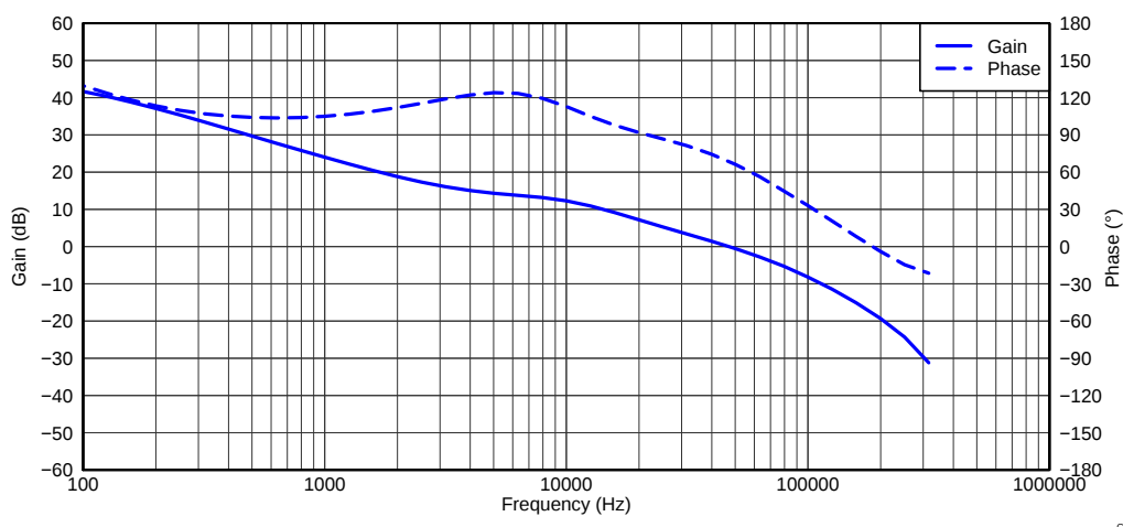
Figure 6. TPS5432EVM-116 Loop Response
