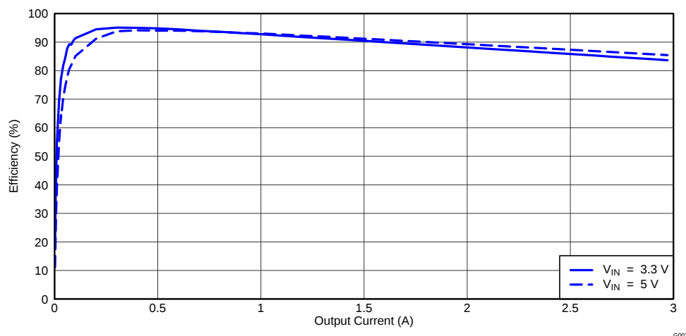
Figure 1. TPS5432EVM-116 Efficiency
