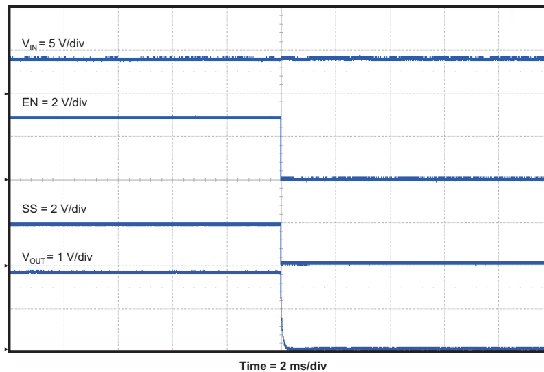
Figure 12. TPS5432EVM-116 Shut Down Relative to EN
