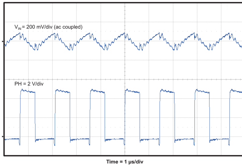
Figure 8. TPS5432EVM-116 Input Ripple
