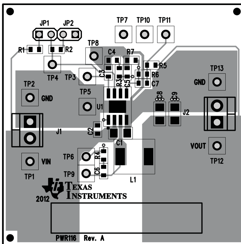
Figure 13. TPS5432EVM-116 Top-Side Assembly
