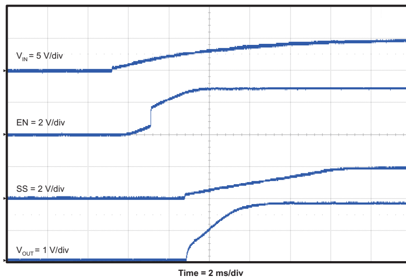
Figure 9. TPS5432EVM-116 Start-Up Relative to V_{IN}
