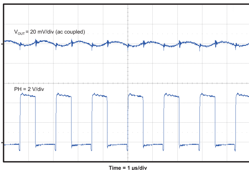
Figure 7. TPS5432EVM-116 Output Ripple
