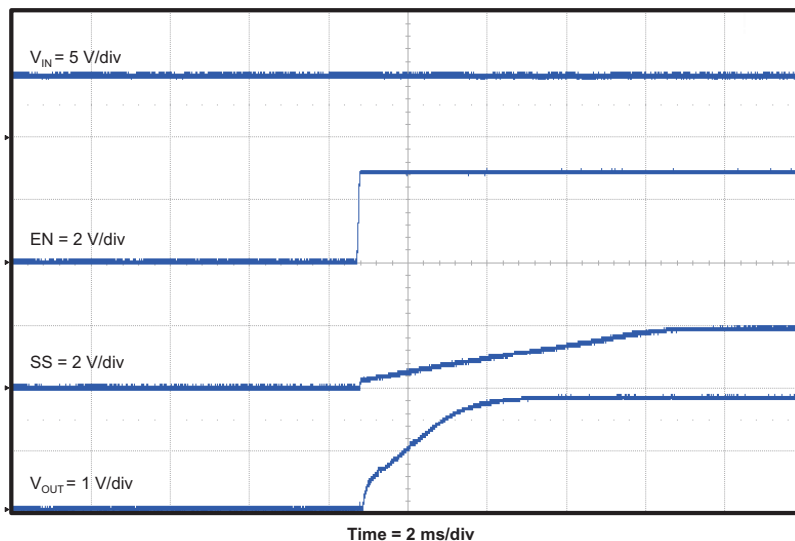
Figure 10. TPS5432EVM-116 Start-Up Relative to EN
