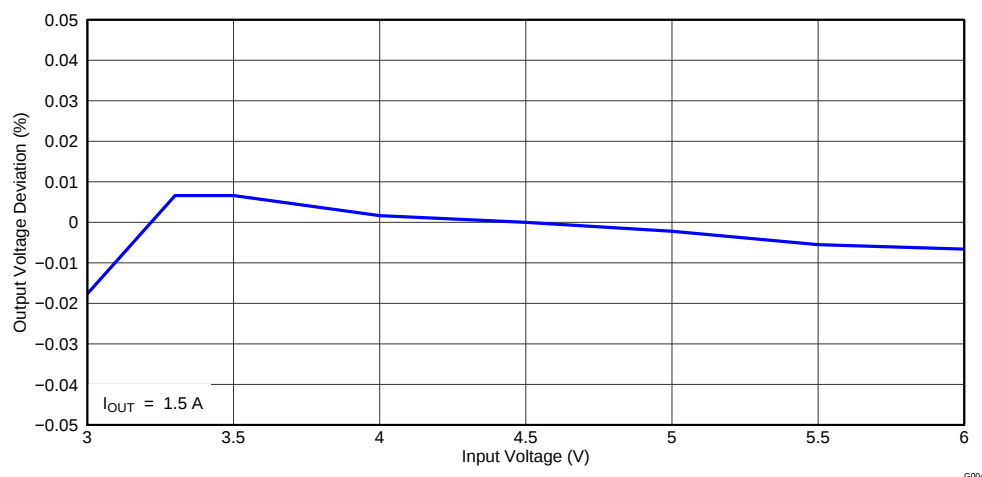
Figure 4. TPS5432EVM-116 Line Regulation
