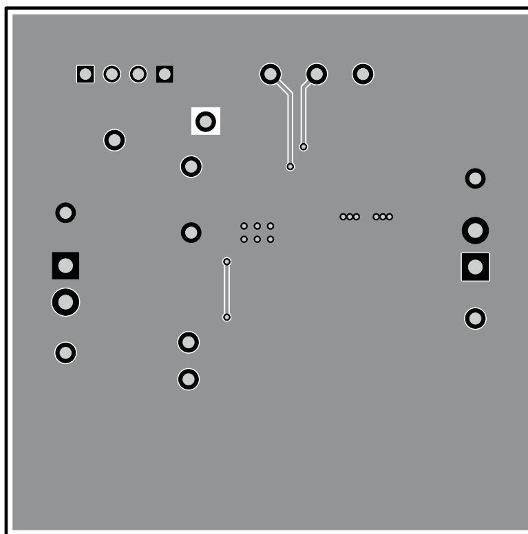
Figure 15. TPS5432EVM-116 Bottom-Side Layout
