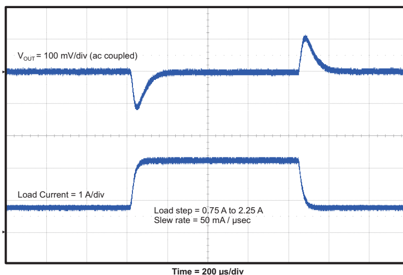
Figure 5. TPS5432EVM-116 Transient Response
