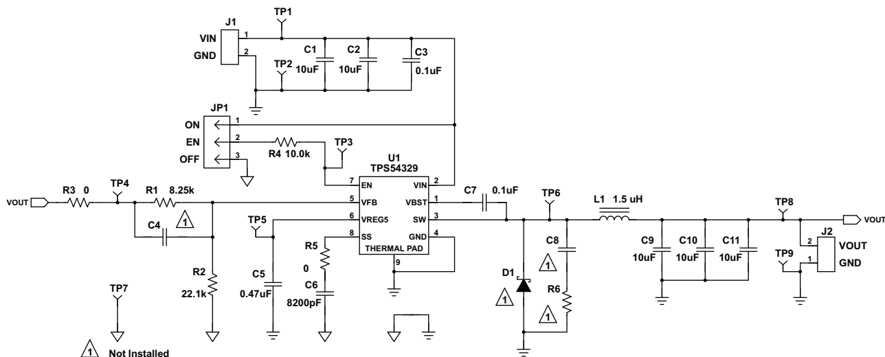
Figure 17. TPS54329EVM-056 Schematic Diagram
