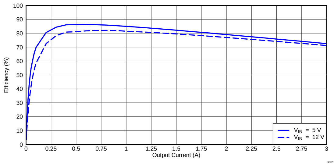
Figure 1. TPS54329EVM-056 Efficiency
