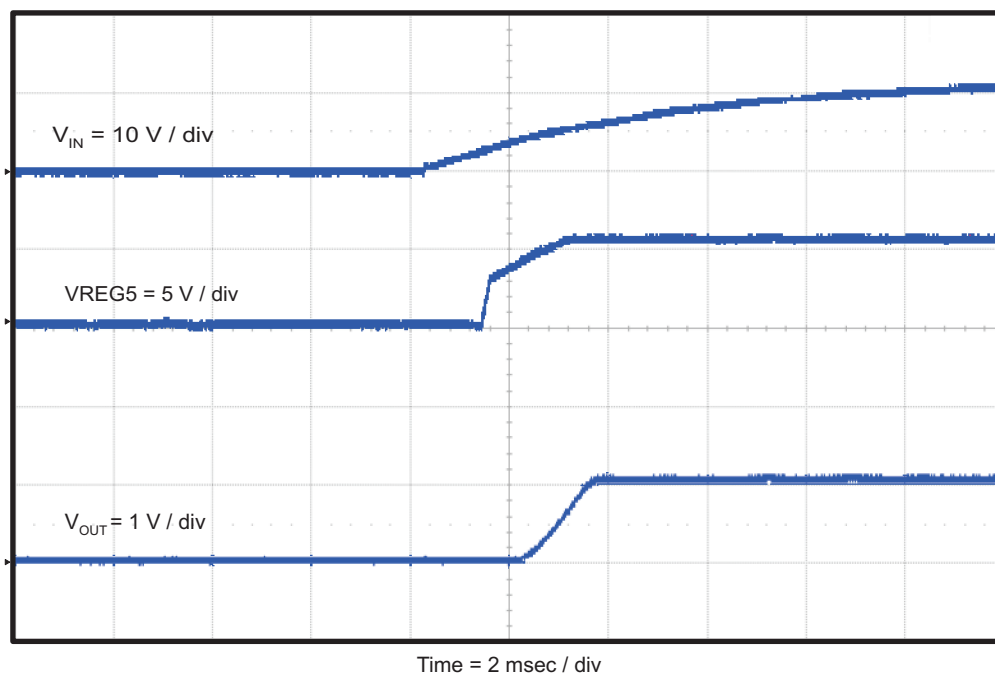
Figure 9. TPS54329EVM-056 Start-Up Relative to V_{IN} With VREG5
