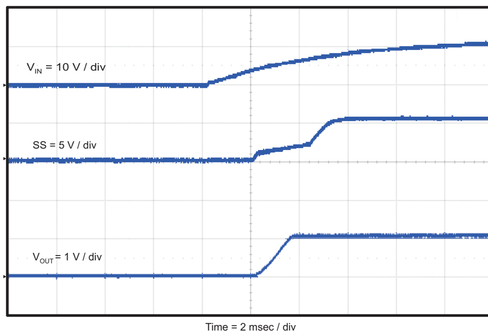
Figure 8. TPS54329EVM-056 Start-Up Relative to V_{IN} With SS
