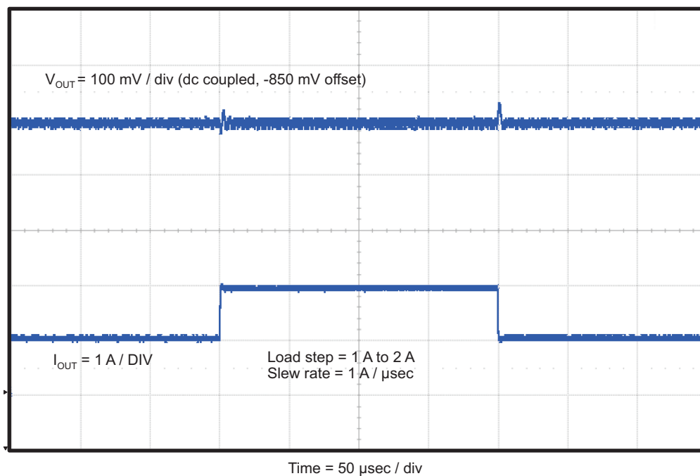
Figure 5. TPS54329EVM-056 Load Transient Response
