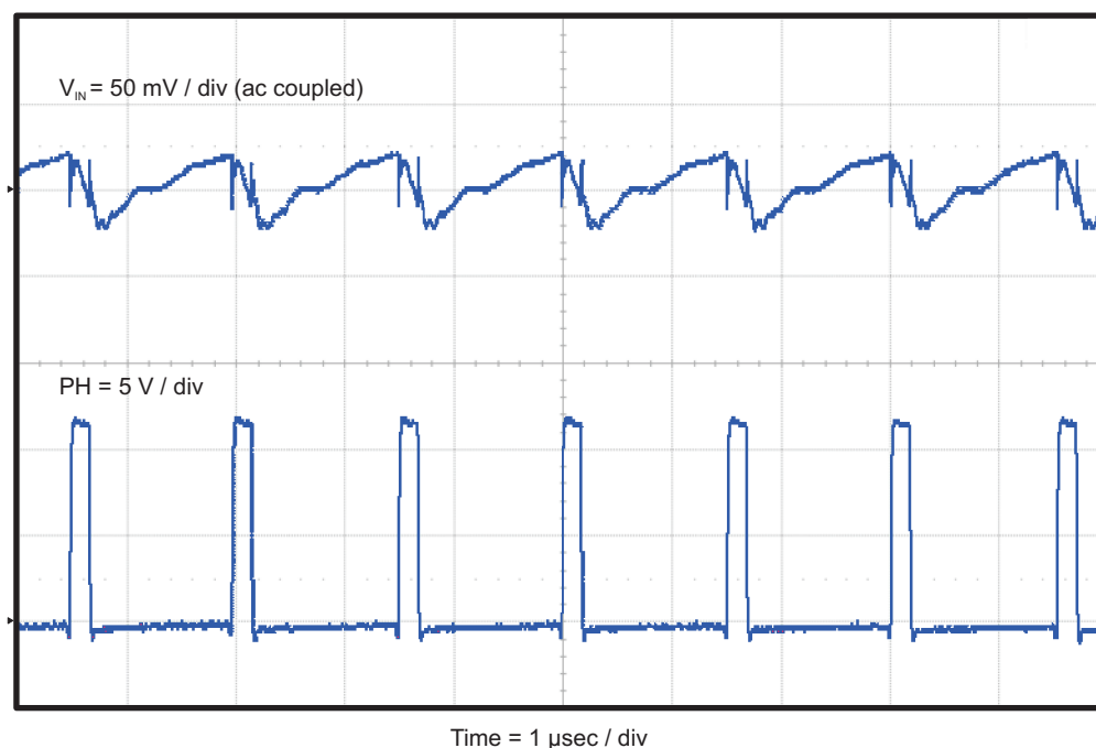
Figure 7. TPS54329EVM-056 Input Voltage Ripple
