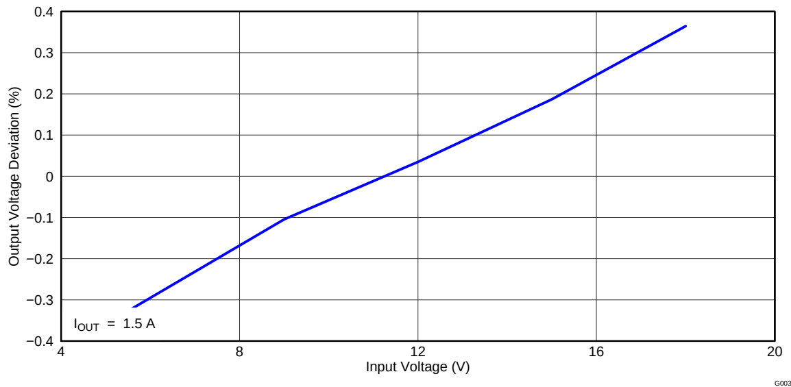
Figure 4. TPS54329EVM-056 Line Regulation
