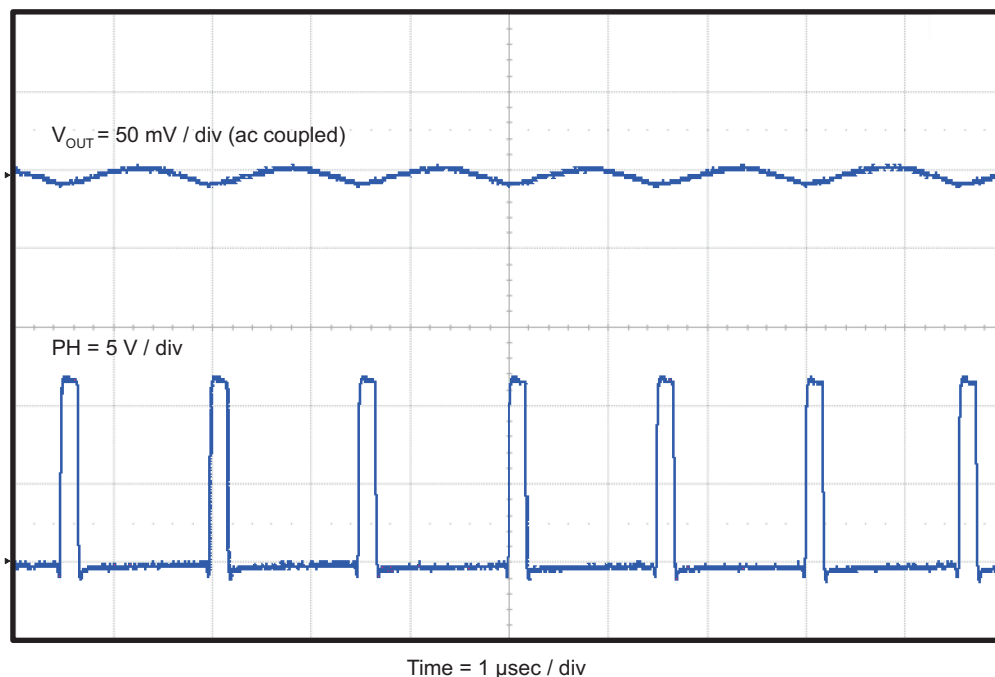
Figure 6. TPS54329EVM-056 Output Voltage Ripple
