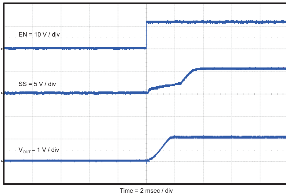
Figure 10. TPS54329EVM-056 Start-Up Relative to EN With SS
