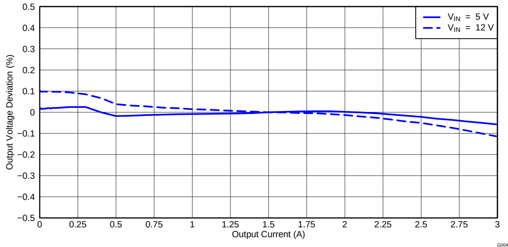
Figure 3. TPS54329EVM-056 Load Regulation, V_{IN} = 5\text{ V}
