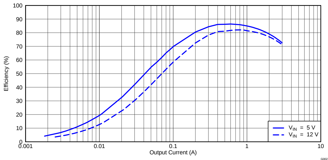
Figure 2. TPS54329EVM-056 Light-Load Efficiency
