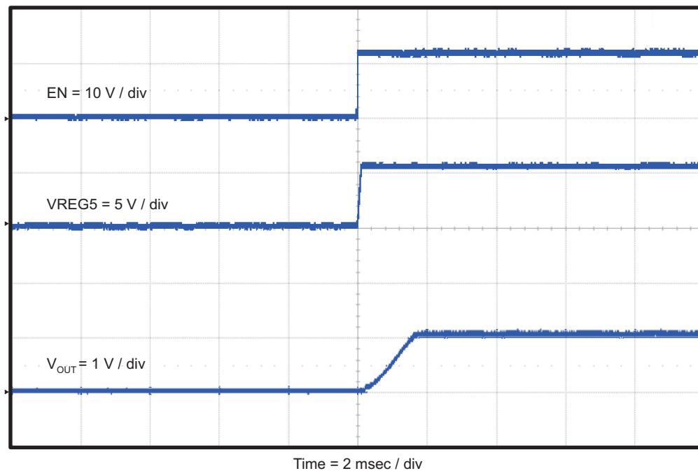
Figure 11. TPS54329EVM-056 Start-Up Relative to EN With VREG5
