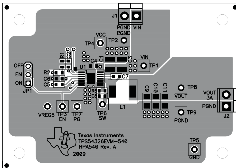
Figure 9. Top Assembly
