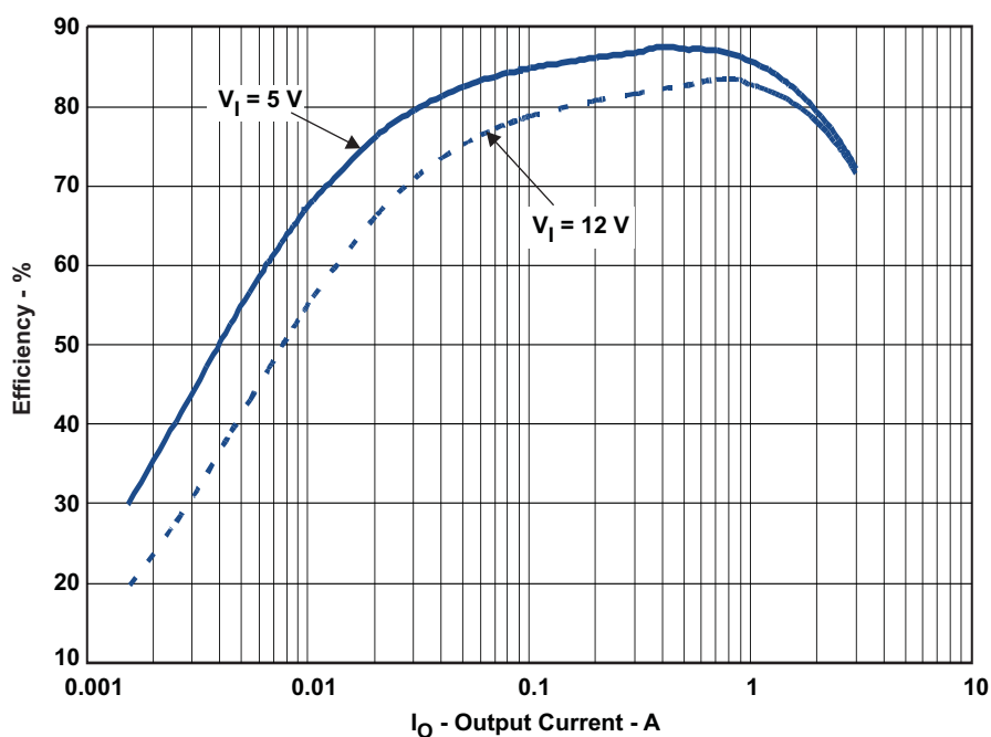
Figure 1. TPS54326EVM-540 Efficiency
