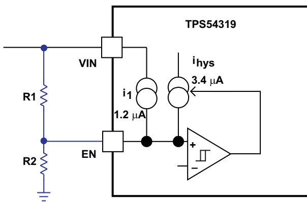
Figure 23. Adjustable Under Voltage Lock Out
