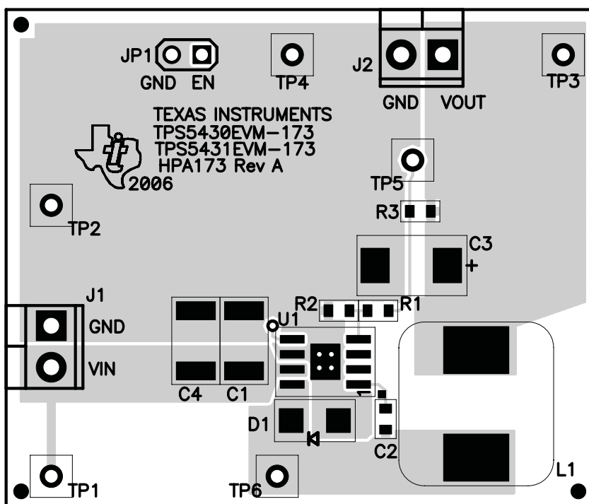
Figure 18. Top-Side Assembly
