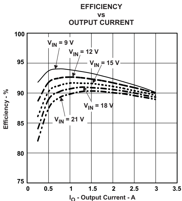
Figure 2. TPS5431 Efficiency
