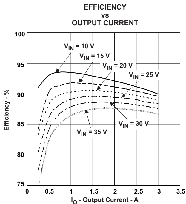
Figure 1. TPS5430 Efficiency
