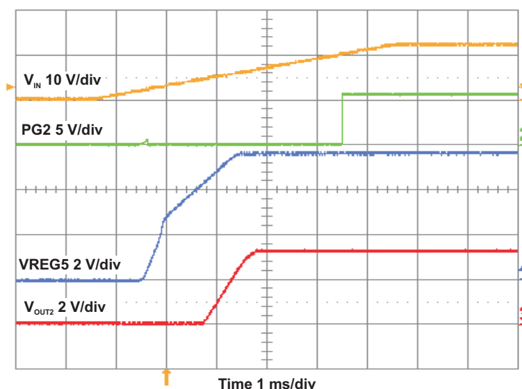
Figure 20. TPS54294EVM Converter 2 Start-Up Relative to V_{IN}
