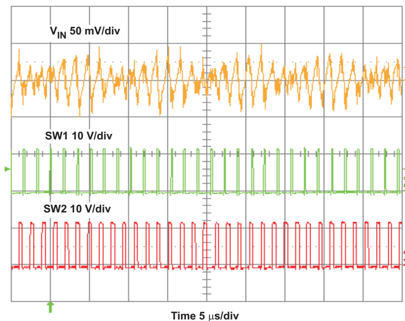
Figure 15. TPS54294EVM Input Voltage Ripple
