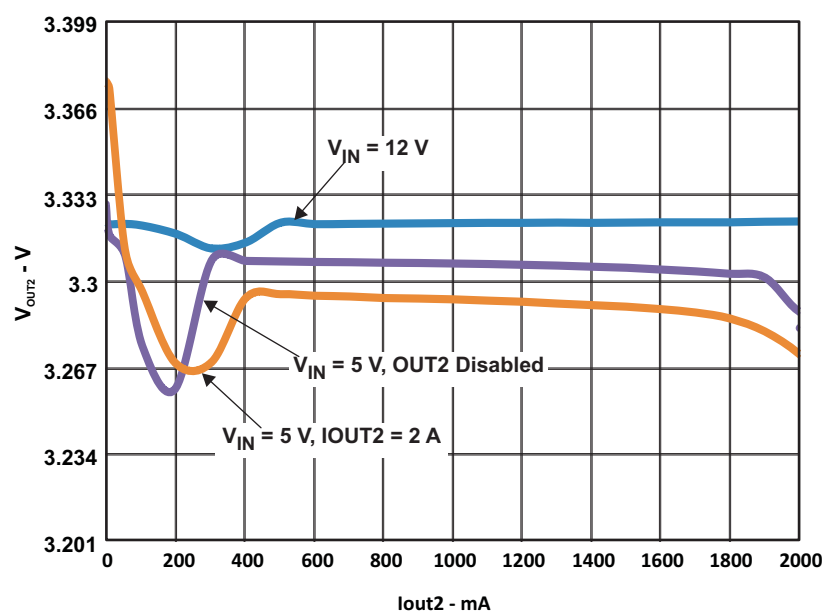
Figure 4. TPS54294EVM Converter 2 Load Regulation
