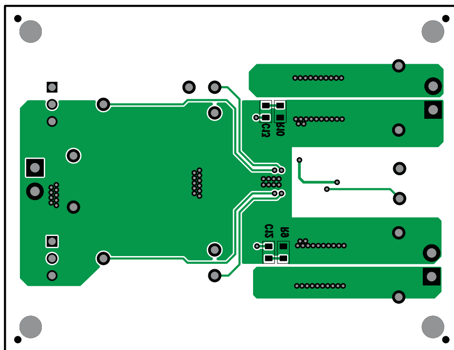
Figure 29. Bottom Assembly
