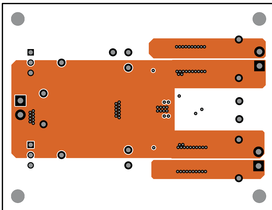
Figure 27. Internal 2 Layer
