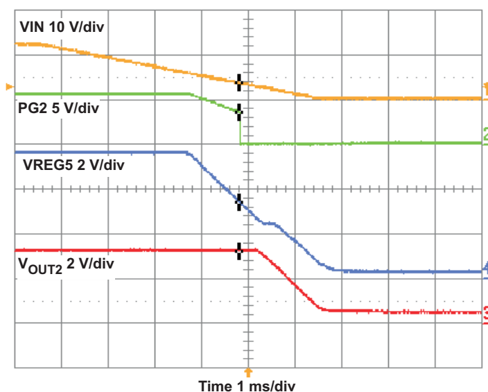
Figure 21. TPS54294EVM Converter 2 Shut-Down Relative to V_{IN}
