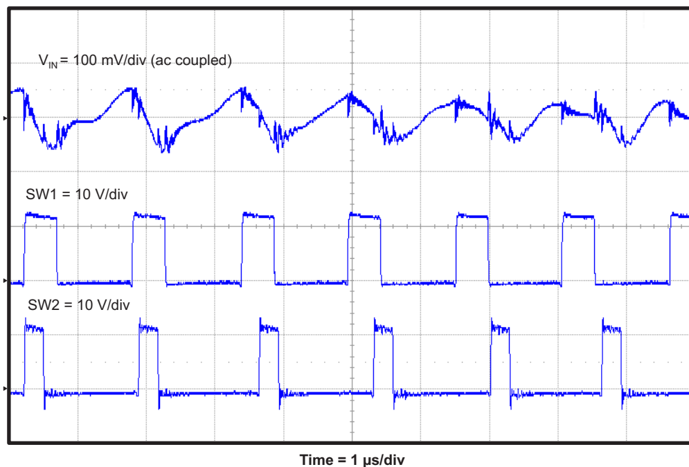
Figure 15. TPS542941EVM Input Voltage Ripple
