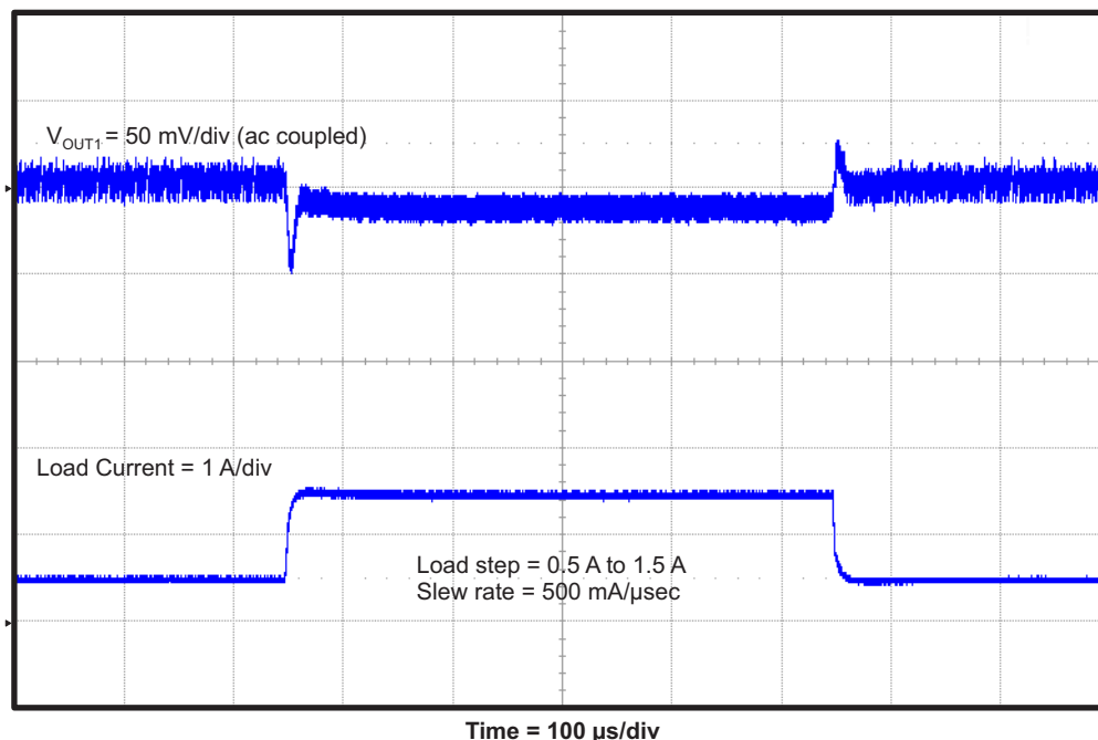
Figure 9. TPS542941EVM Converter 1 Load Transient Response
