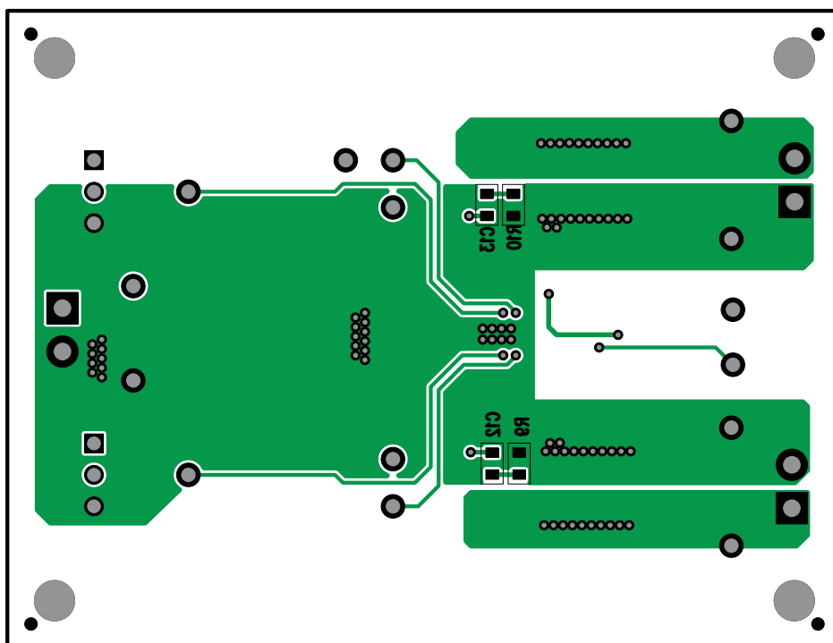
Figure 25. Bottom Assembly
