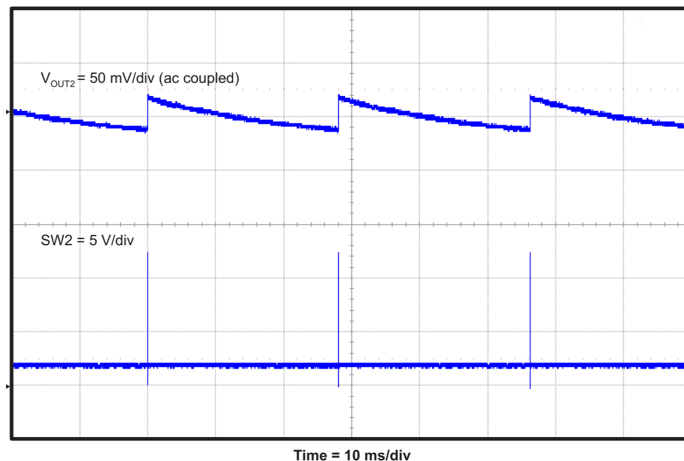
Figure 14. TPS542941EVM Converter 2 Eco-mode™ Output Voltage Ripple at No Load
