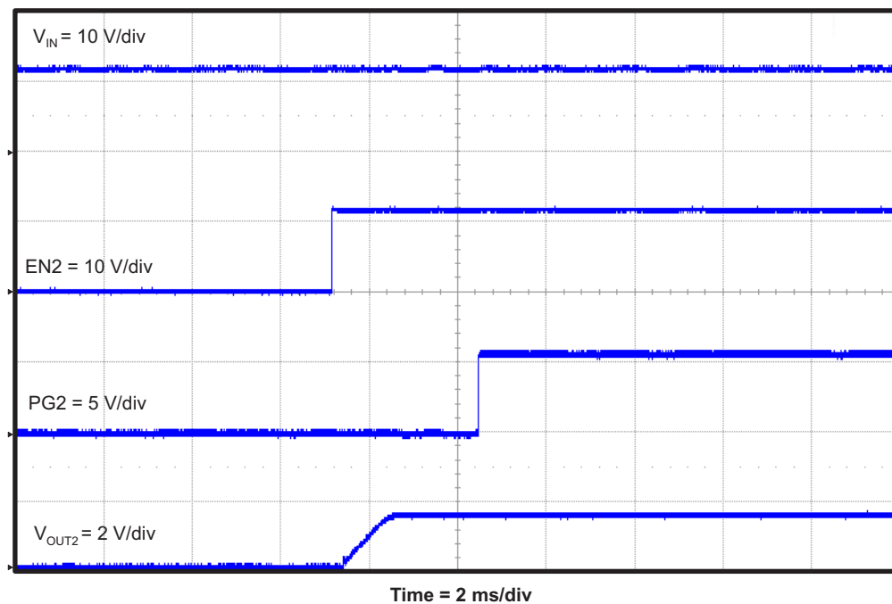
Figure 19. TPS542941EVM Start-Up Relative to EN2
