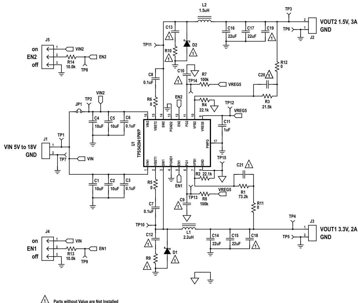
Figure 26. TPS542941EVM Schematic Diagram
