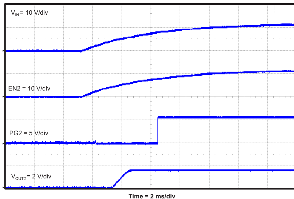
Figure 18. TPS542941EVM Converter 2 Start-Up Relative to V_{IN}
