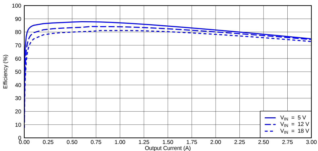
Figure 3. TPS542941EVM Converter 2 Efficiency
