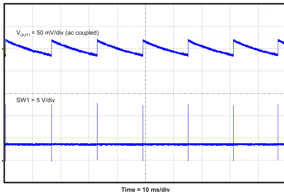
Figure 12. TPS542941EVM Converter 1 Eco-mode™ Output Voltage Ripple at No Load
