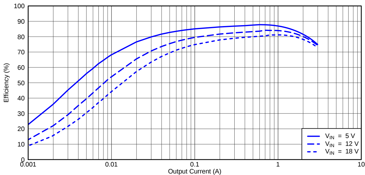
Figure 4. TPS542941EVM Converter 2 Light Load Efficiency
