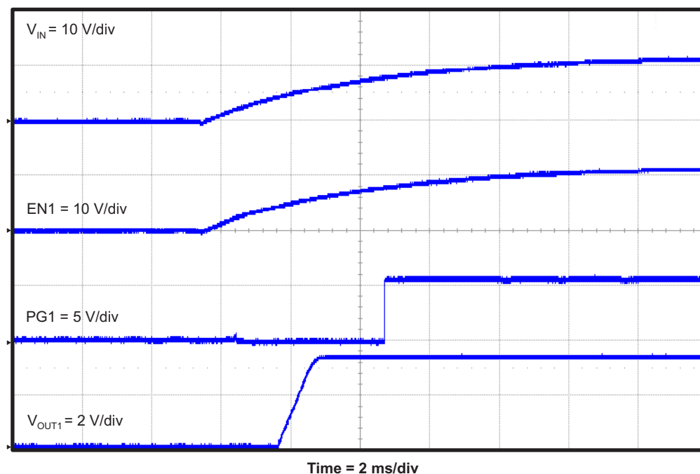
Figure 16. TPS542941EVM Converter 1 Start-Up Relative to V_{IN}
