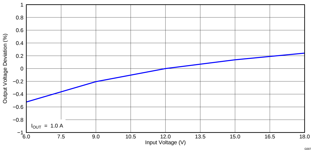
Figure 7. TPS542941EVM Converter 1 Line Regulation
