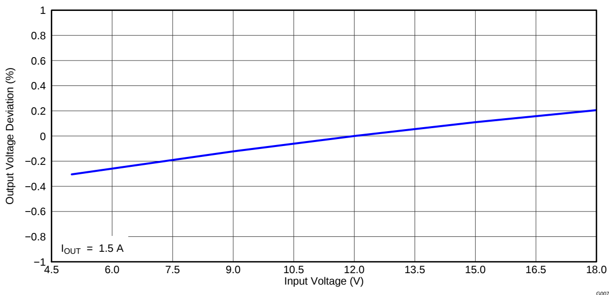
Figure 8. TPS542941EVM Converter 2 Line Regulation
