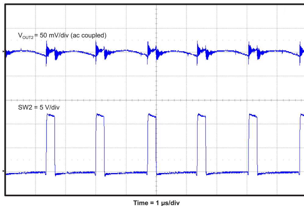
Figure 13. TPS542941EVM Converter 2 Output Voltage Ripple
