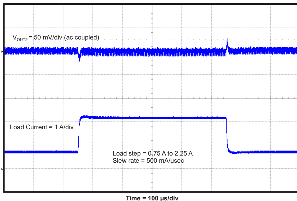
Figure 10. TPS542941EVM Converter 2 Load Transient Response
