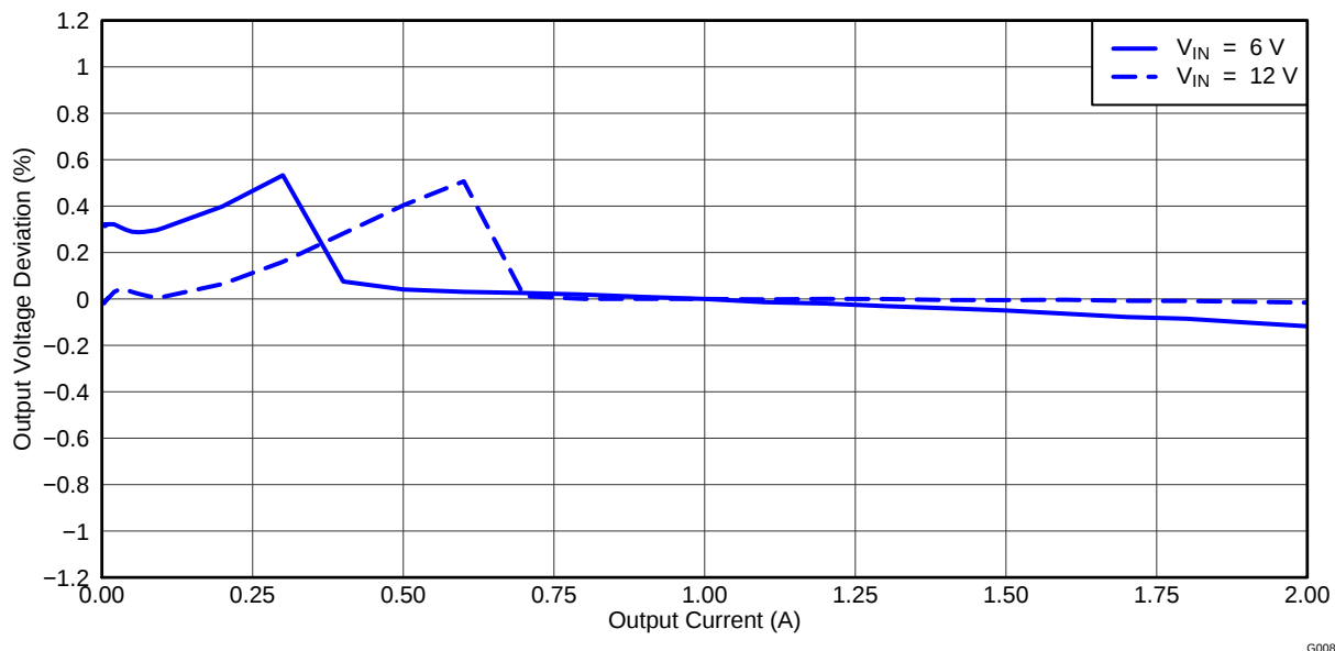
Figure 5. TPS542941EVM Converter 1 Load Regulation
