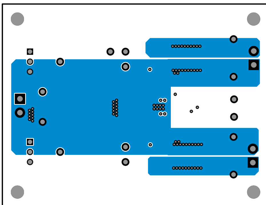
Figure 22. Internal 1 Layer
