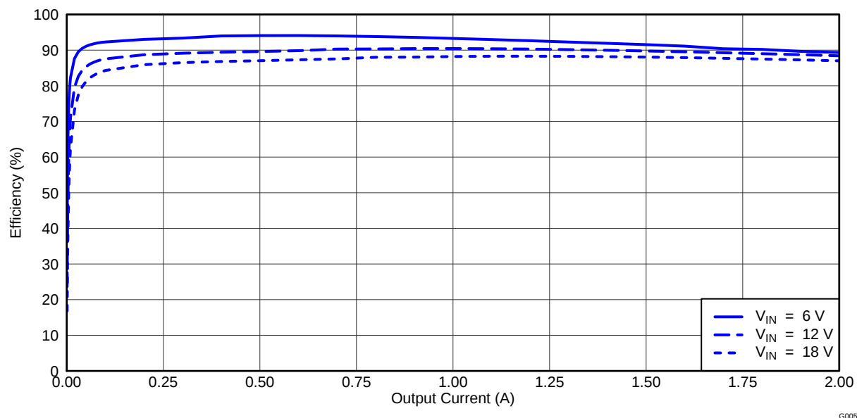
Figure 1. TPS542941EVM Converter 1 Efficiency
