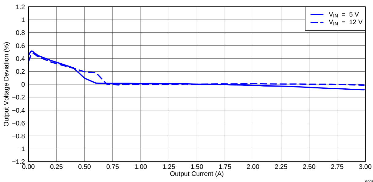
Figure 6. TPS542941EVM Converter 2 Load Regulation
