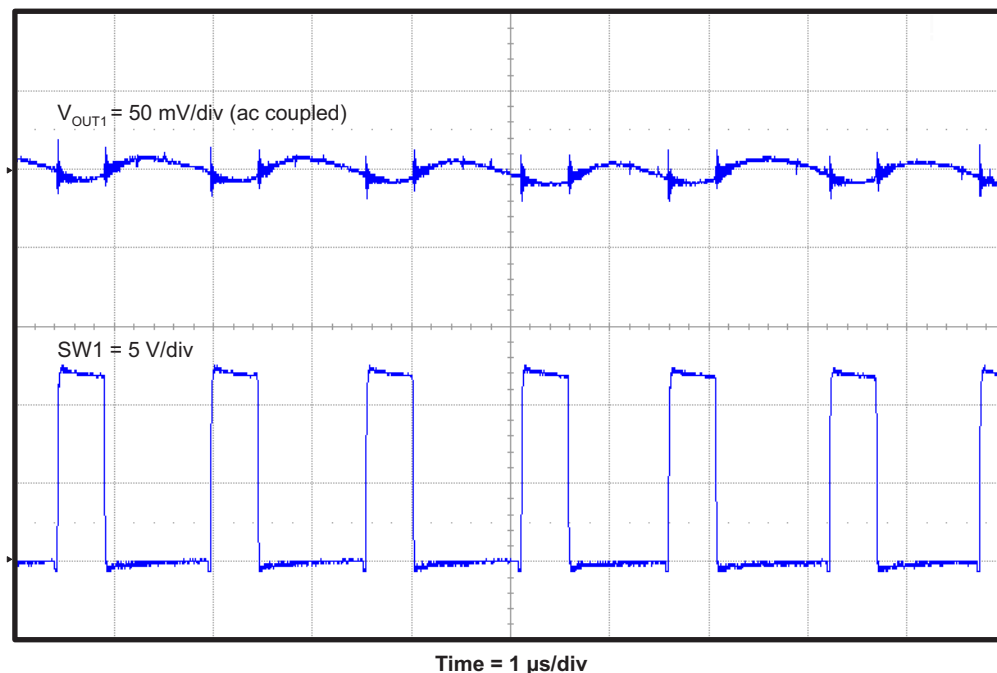
Figure 11. TPS542941EVM Converter 1 Output Voltage Ripple
