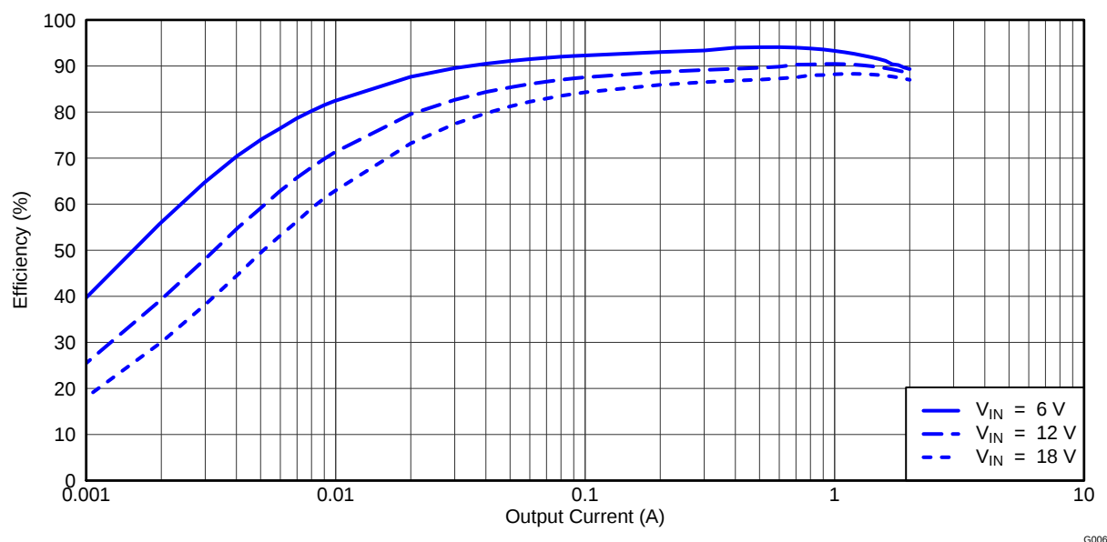
Figure 2. TPS542941EVM Converter 1 Light Load Efficiency
