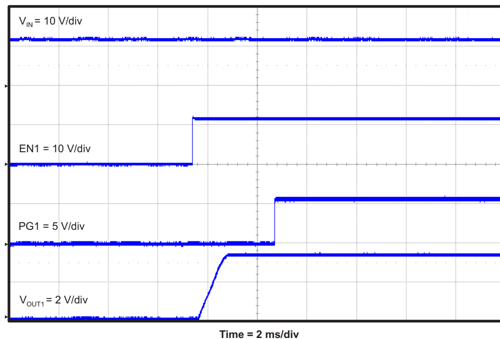
Figure 17. TPS542941EVM Start-Up Relative to EN1
