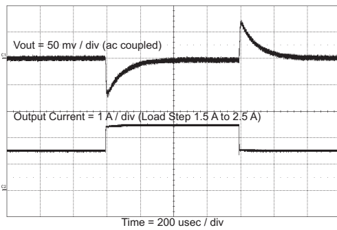
Figure 51. Load Transient
