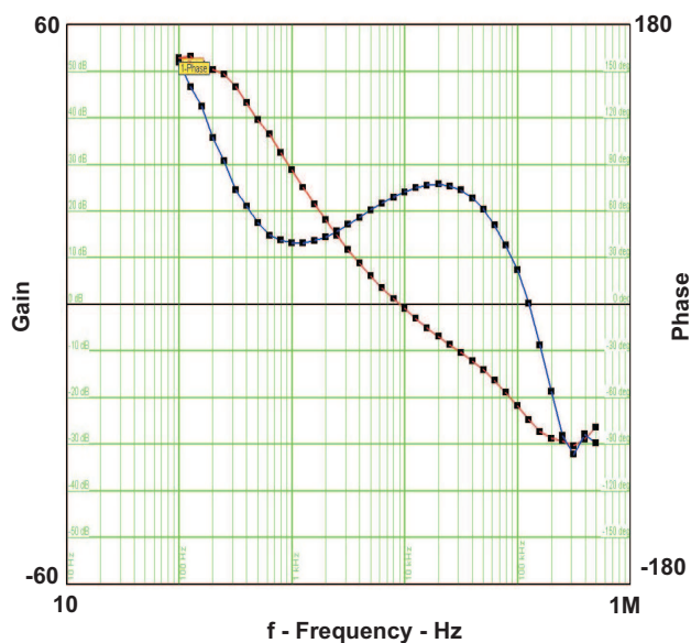
Figure 6. TPS54233EVM-373 Loop Response
