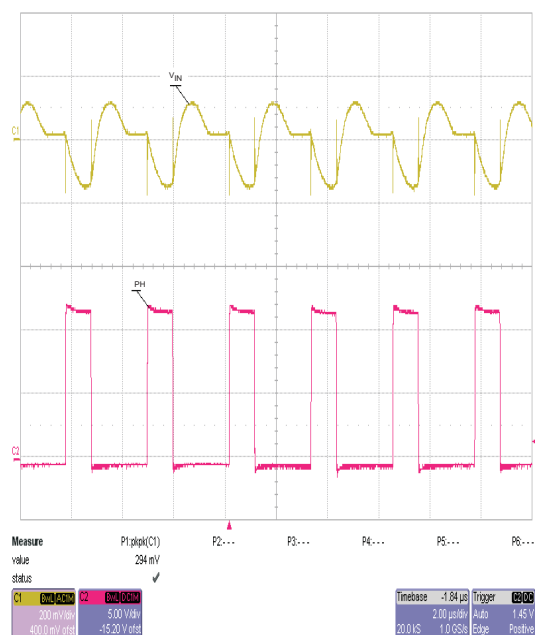
Figure 8. TPS54233EVM-373 Input Ripple
