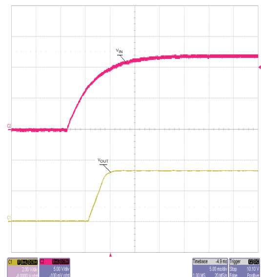
Figure 9. TPS54233EVM-373 Start-Up Relative to V_{IN}
