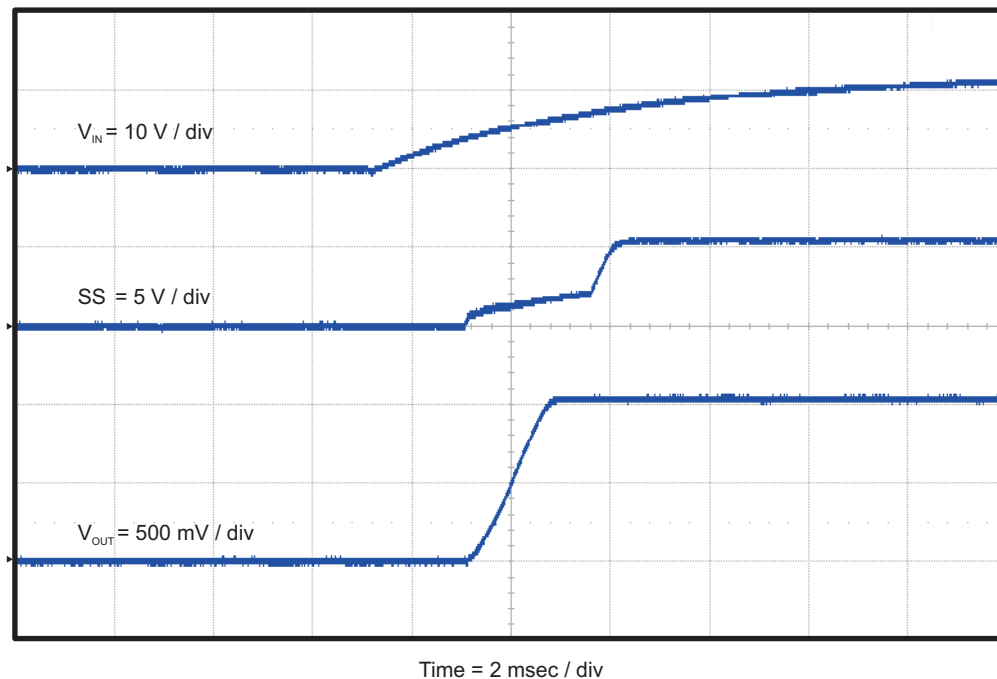
Figure 9. TPS54227EVM-686 Start-Up Relative to V_{IN}
