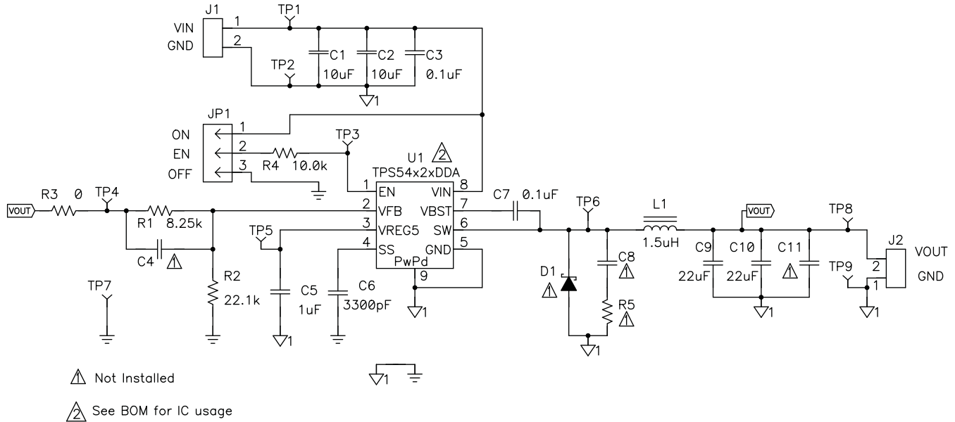
Figure 15. TPS54227EVM-686 Schematic Diagram
