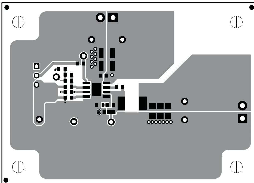
Figure 12. Top Layer
