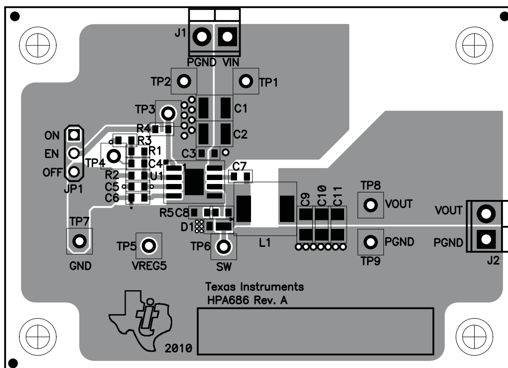
Figure 11. Top Assembly
