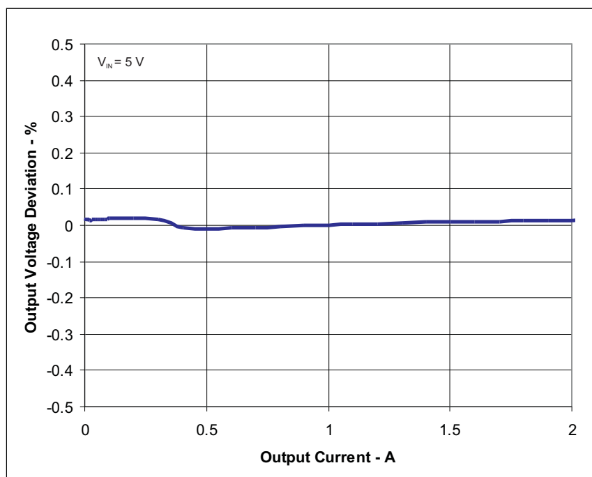
Figure 3. TPS54227EVM-686 Load Regulation, V_{IN} = 5 V.
