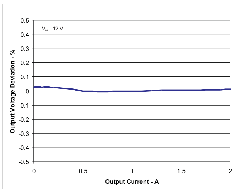
Figure 4. TPS54227EVM-686 Load Regulation, V_{IN} = 12 V.
