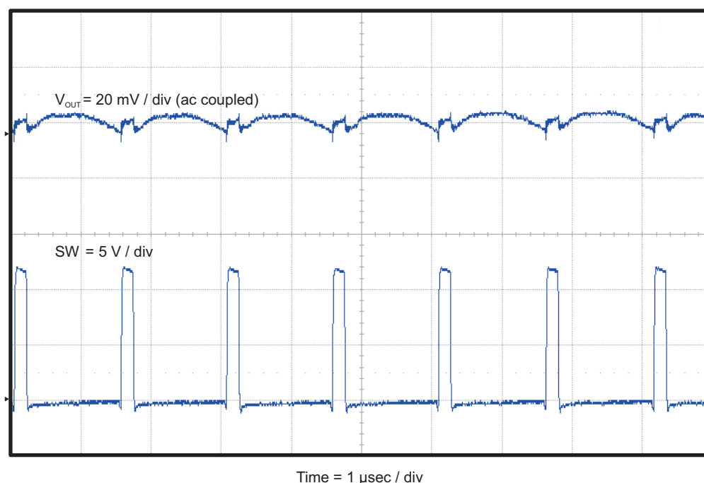
Figure 7. TPS54227EVM-686 Output Voltage Ripple
