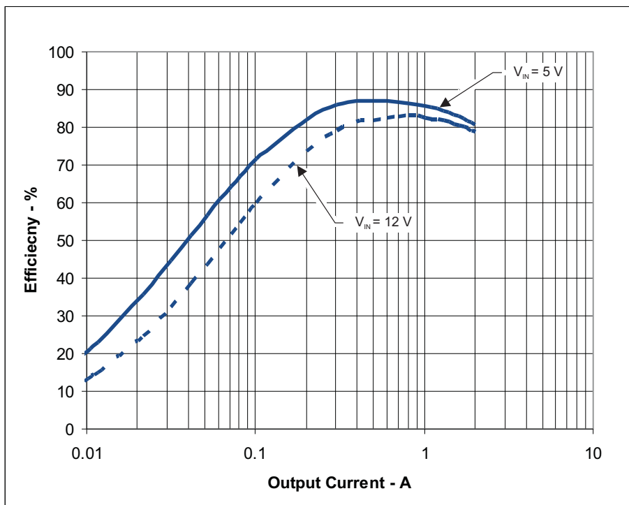
Figure 2. TPS54227EVM-686 Light Load Efficiency
