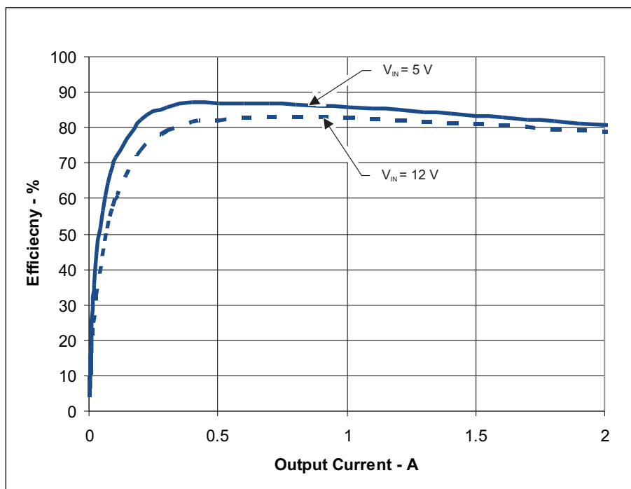
Figure 1. TPS54227EVM-686 Efficiency
