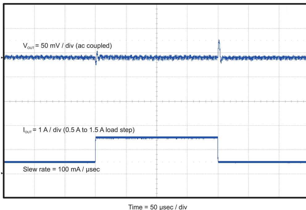
Figure 6. TPS54227EVM-686 Load Transient Response
