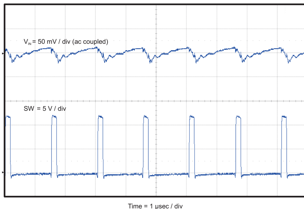
Figure 8. TPS54227EVM-686 Input Voltage Ripple
