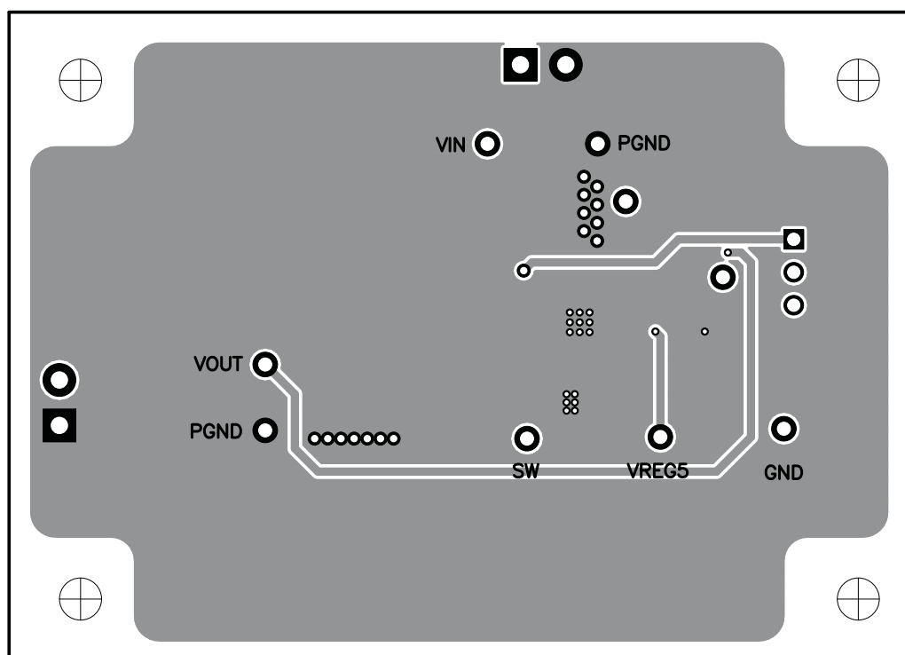
Figure 14. Bottom Assembly
