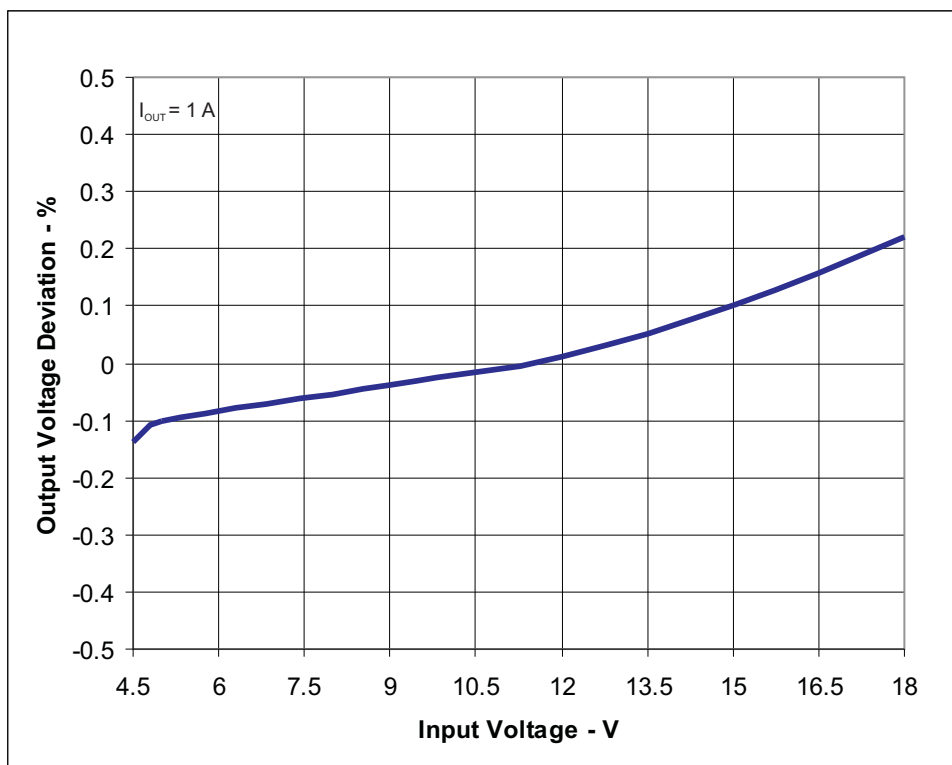
Figure 5. TPS54227EVM-686 Line Regulation
