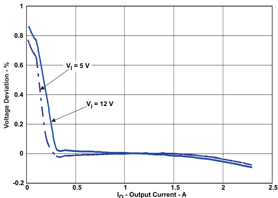
Figure 2. TPS54226EVM-539 Load Regulation
