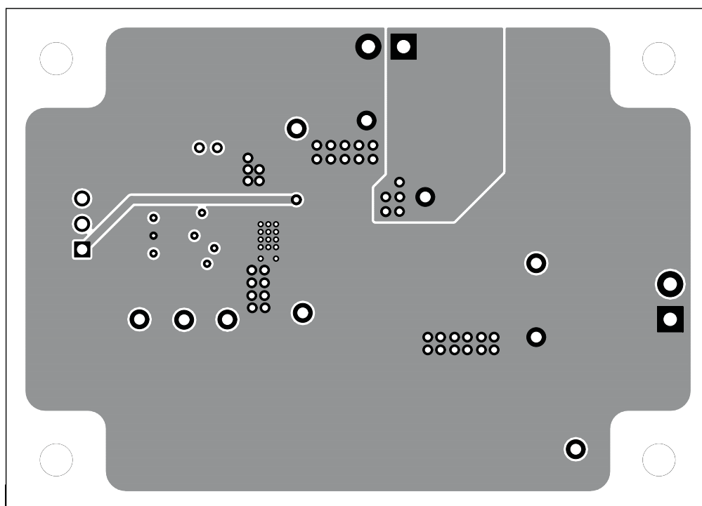
Figure 12. Internal Layer 2
