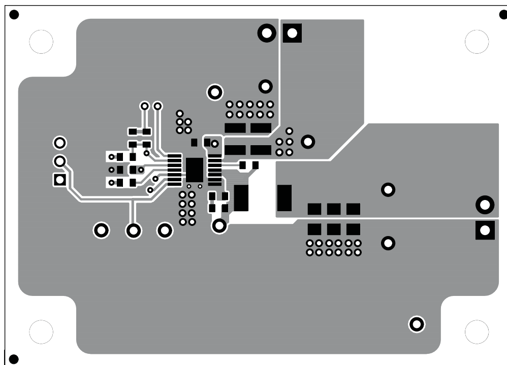
Figure 10. Top Layer
