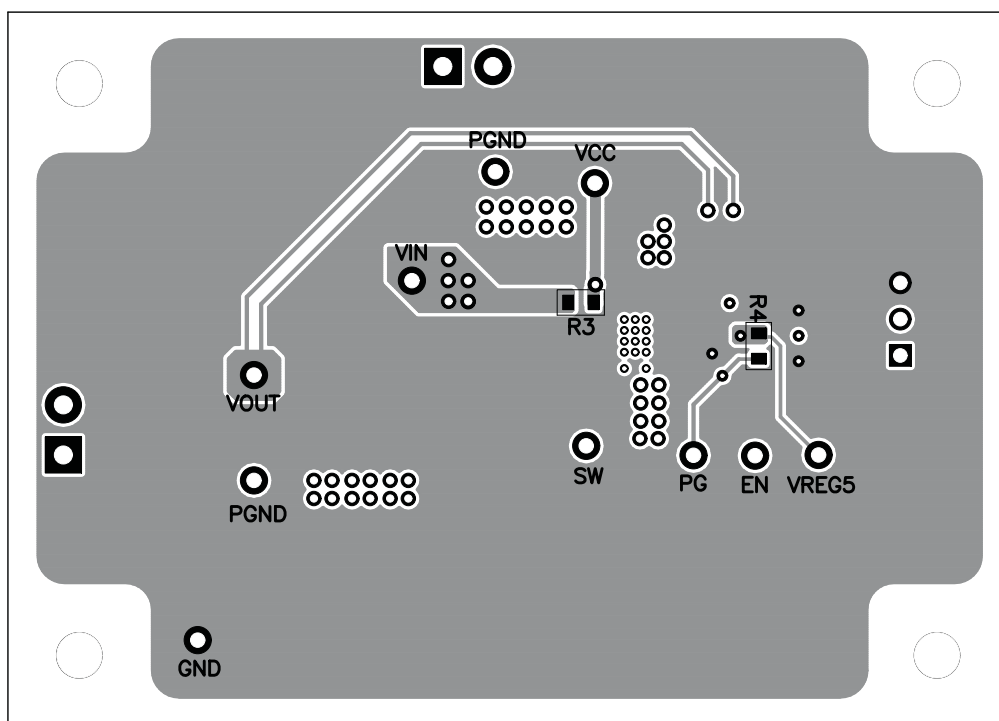
Figure 14. Bottom Assembly
