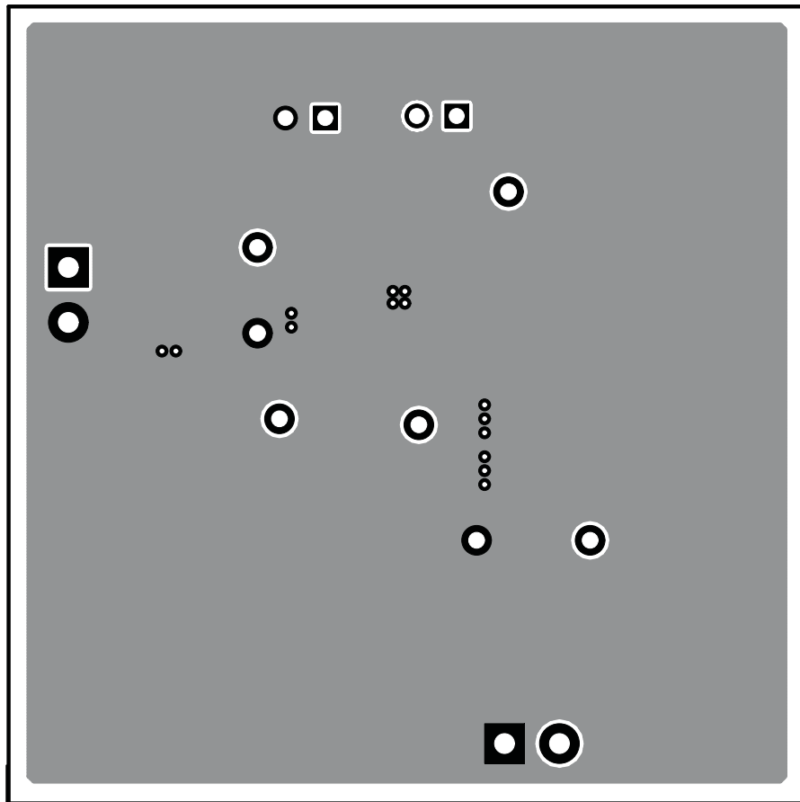
Figure 13. TPS54218EVM-511 Layout 2
