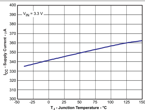
Figure 18. Supply Current versus Junction Temperature
