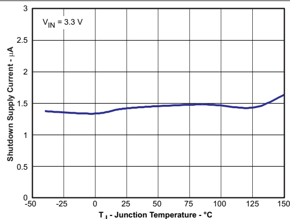
Figure 16. Shutdown Supply Current versus Junction Temperature
