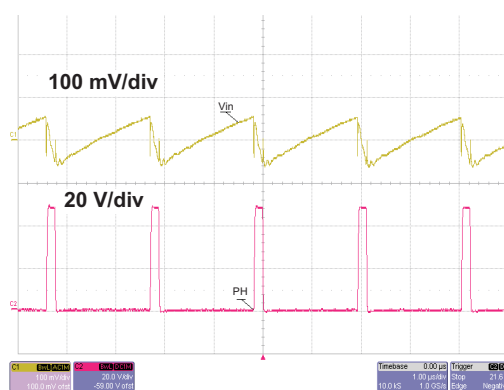
Figure 9. Bottom Converter Input Voltage Ripple, Vin=48.0V, Iout=1.5A
