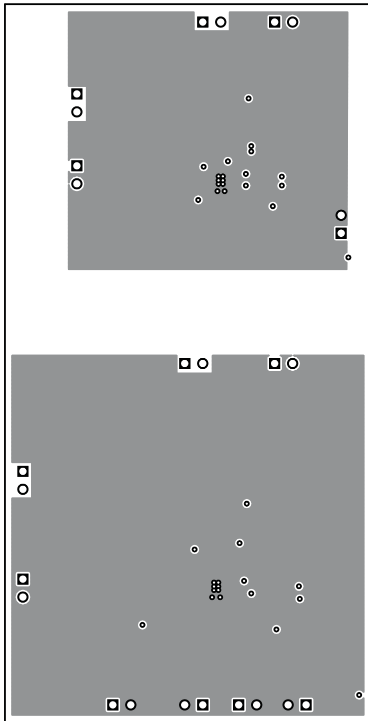
Figure 19. Layer 3 Routing
