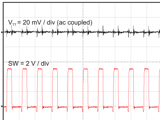
Time = 500 nsec / div Figure 60. V_{TT} Output Ripple
