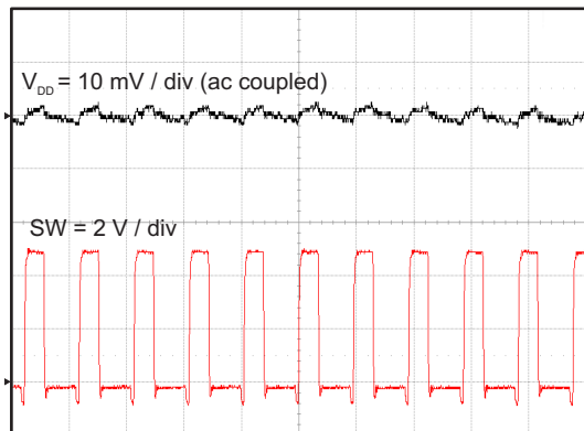
Time = 500 nsec / div Figure 59. V_{DD} Output Ripple
